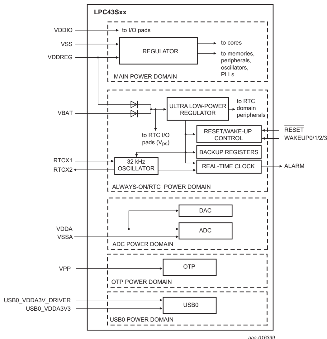
Fig 7. Power domains
