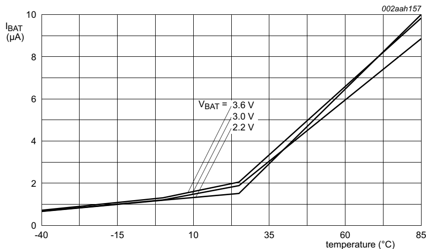
Fig 16. Typical battery supply versus temperature in Deep power-down mode
