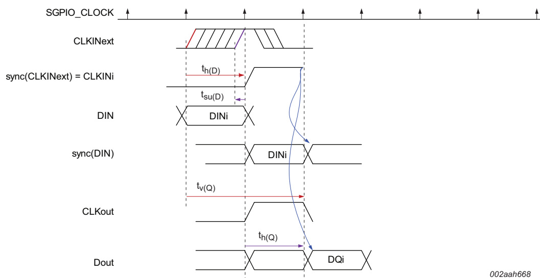
Fig 31. SGPIO timing
