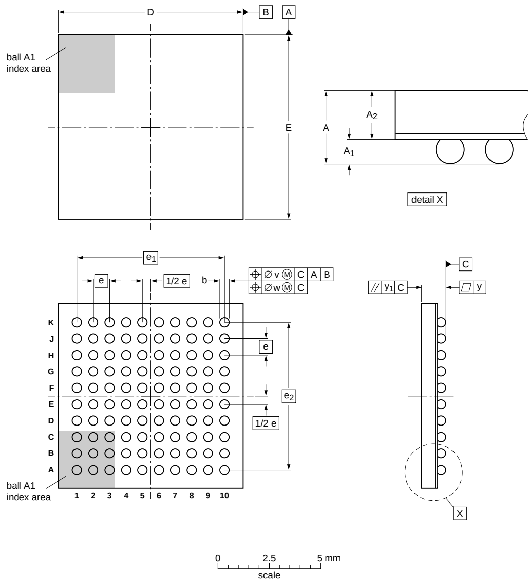
TFBGA100: plastic thin fine-pitch ball grid array package; 100 balls; body 9 x 9 x 0.7 mm
