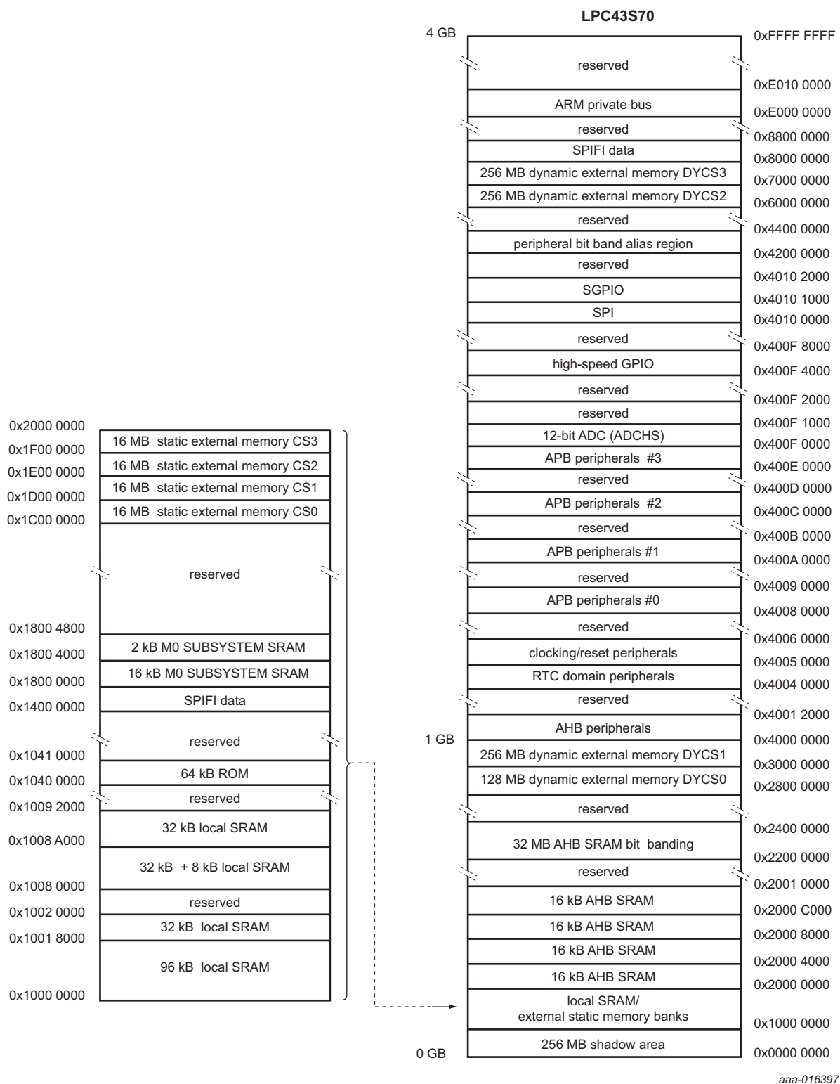
Fig 5. LPC43S70 Memory mapping (overview)
