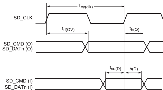
Fig 39. SD/MMC timing
