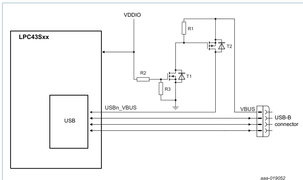
Fig 49. USB interface for USB operating in OTG mode
