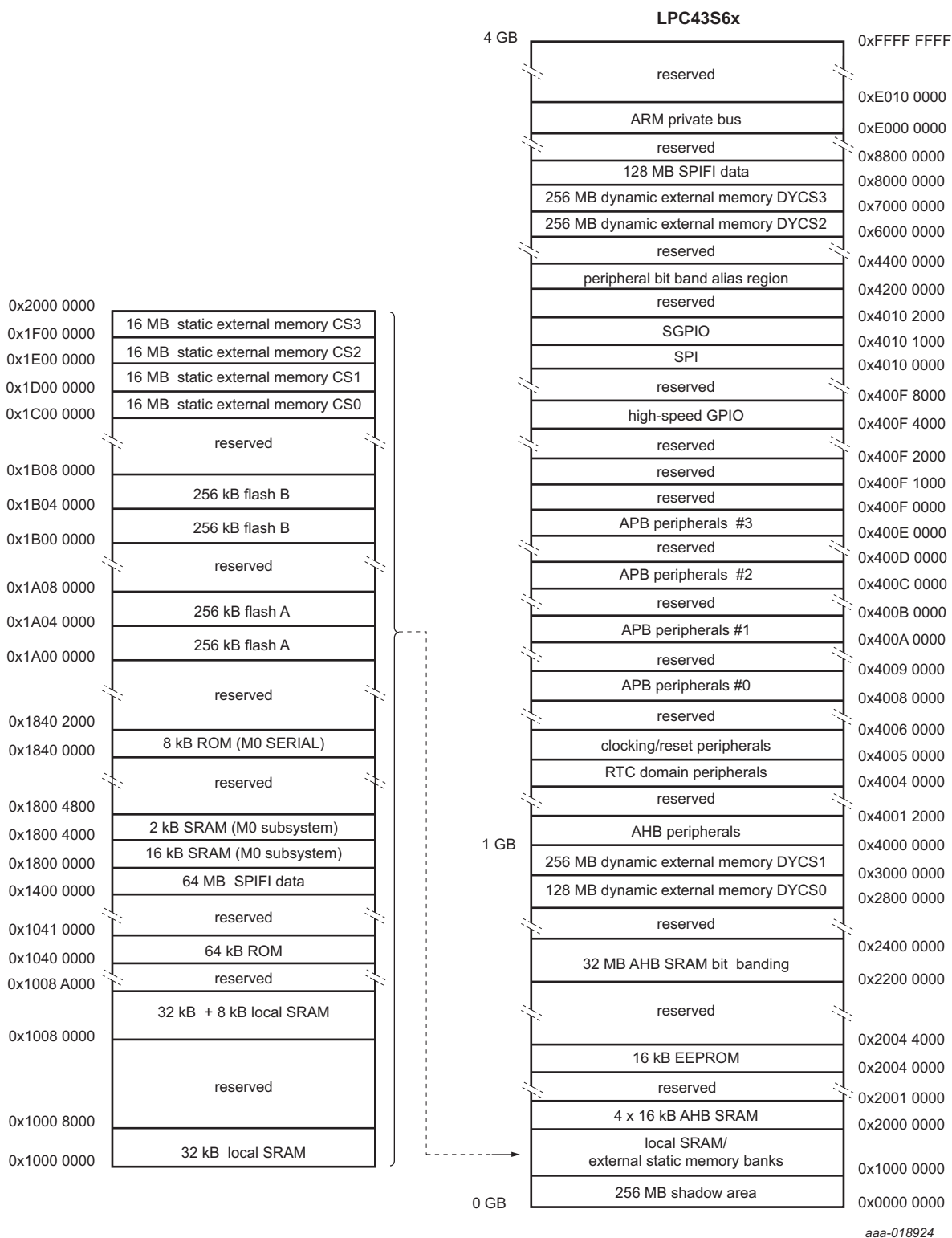
Fig 6. LPC43S6x Memory mapping (overview)
