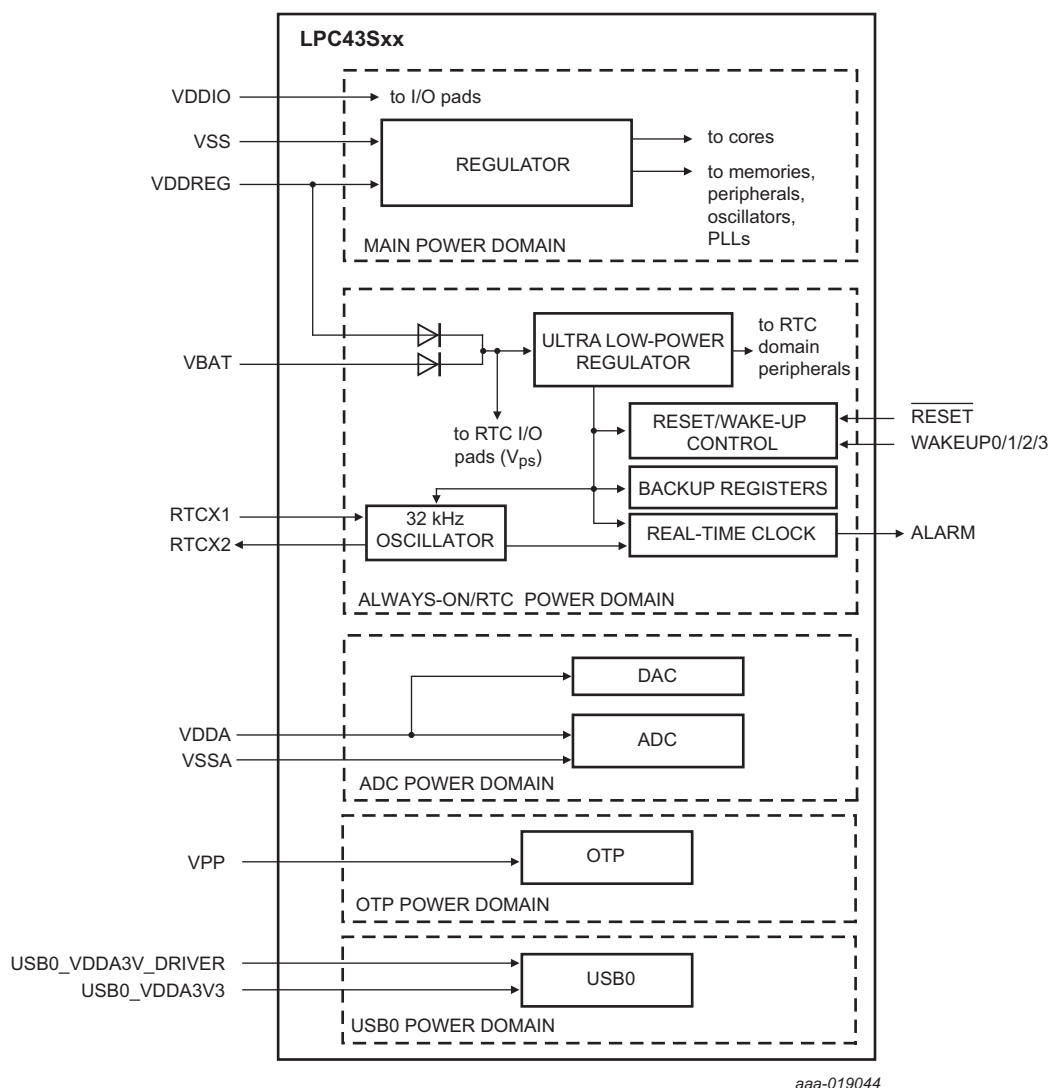
Fig 8. Power domains
