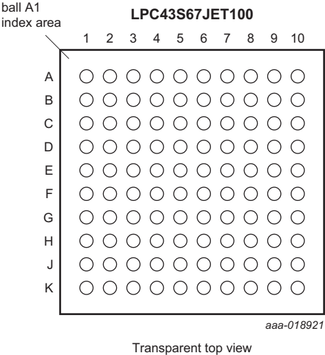
Fig 3. Pin configuration LQFP100 package
