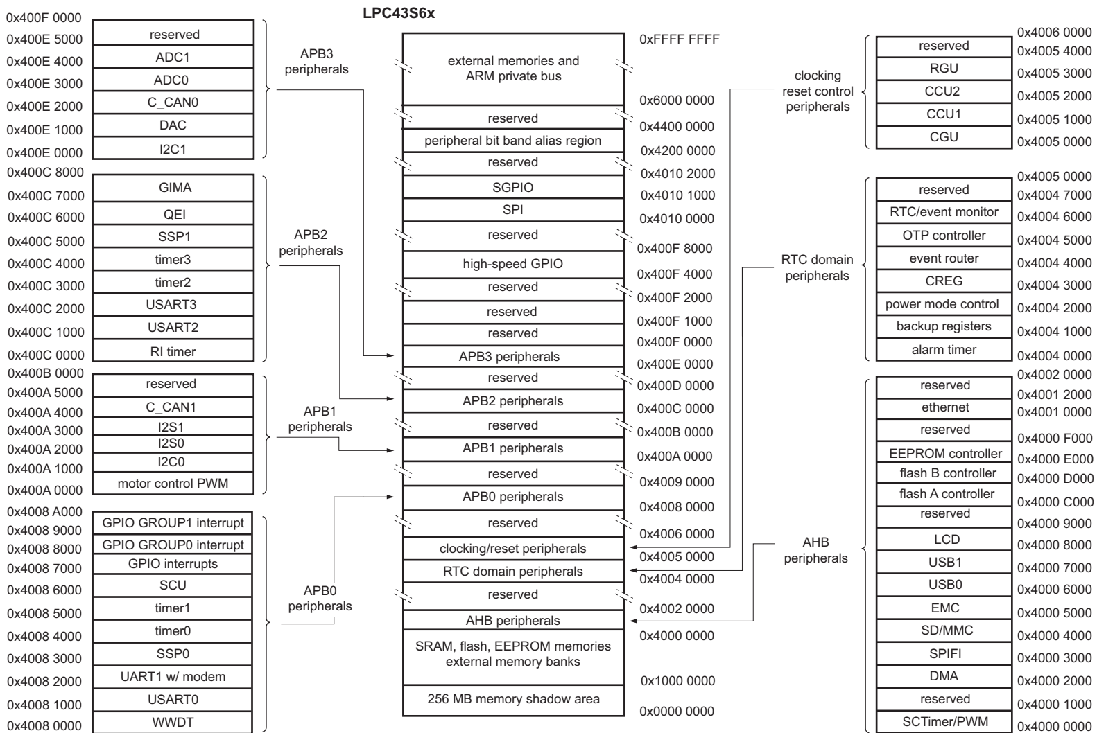
Fig 7. LPC43S6x Memory mapping (peripherals)
