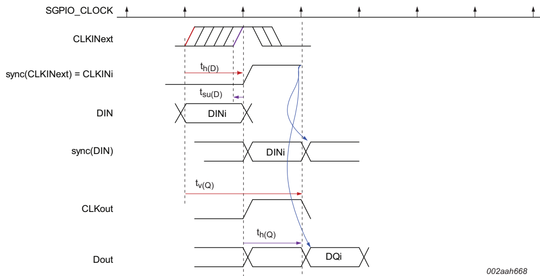
Fig 31. SGPIO timing
