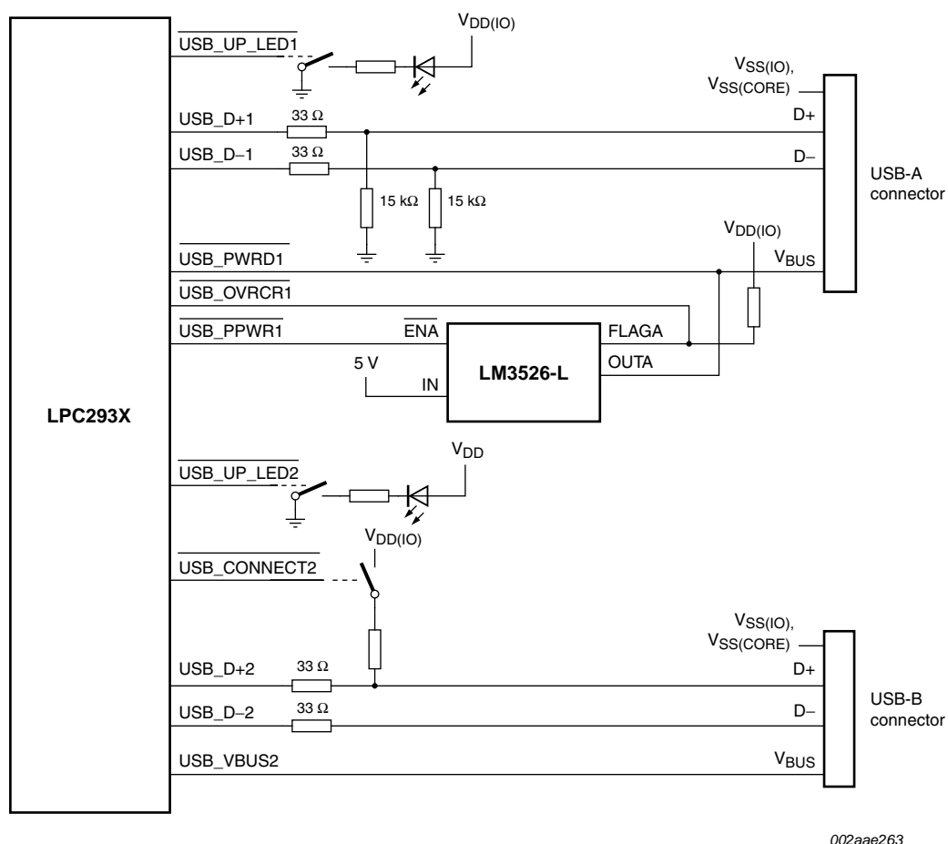
Fig 36. LPC2930 USB OTG port configuration: USB port 2 device, USB port 1 host
