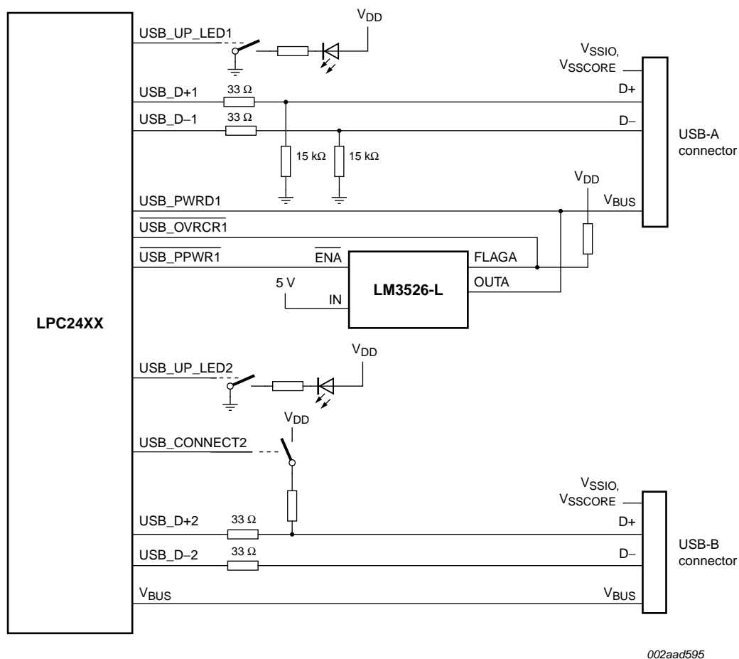
Fig 25. LPC2478 USB OTG port configuration: USB port 2 device, USB port 1 host
