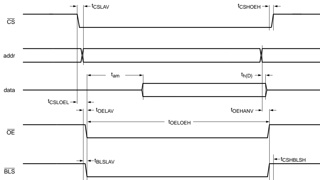
Fig 14. External memory read access
