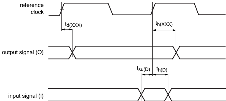
Fig 18. Signal timing
