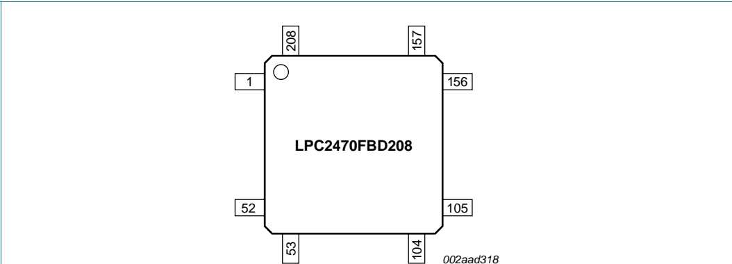
Fig 2. LPC2470 pinning LQFP208 package
