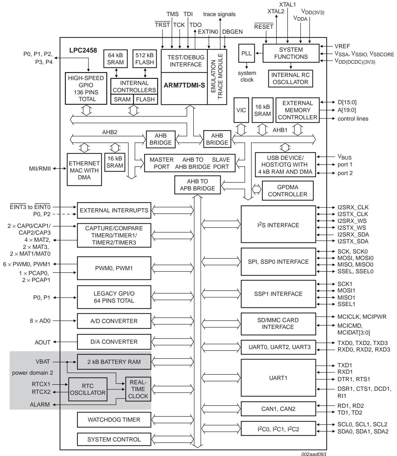
Fig 1. LPC2458 block diagram
