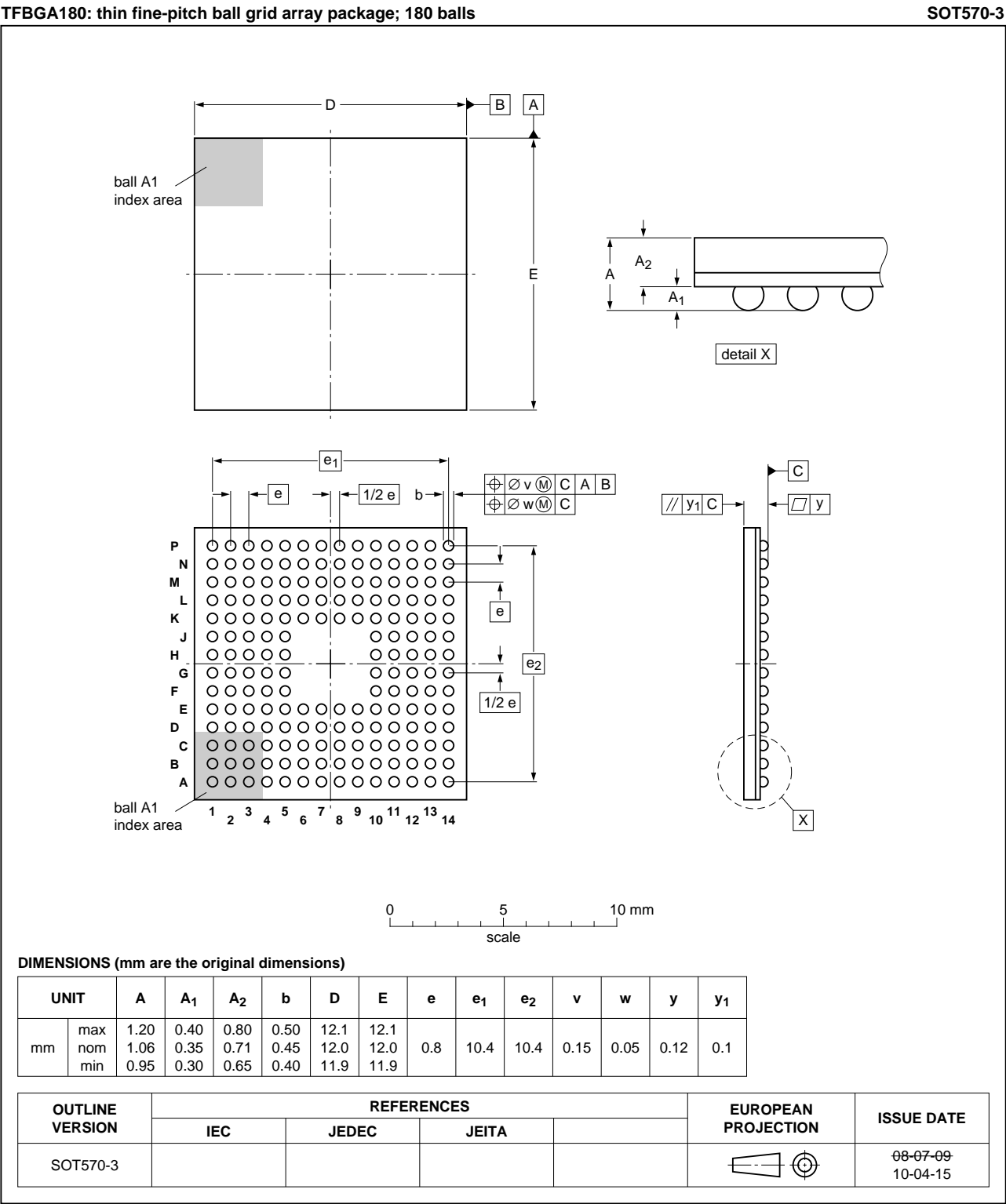
Fig 31. Package outline SOT570-3 (TFBGA180)
