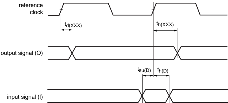
Fig 17. Signal timing
