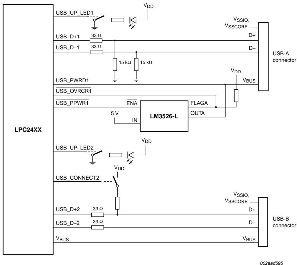
Fig 24. LPC2458 USB OTG port configuration: USB port 2 device, USB port 1 host
