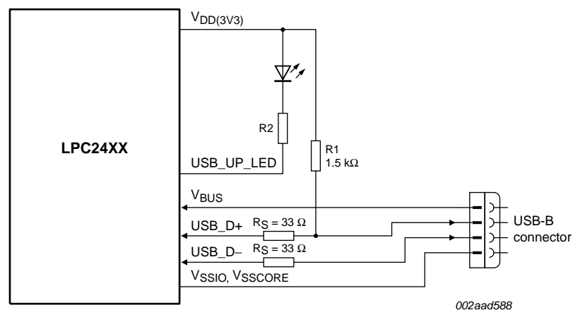
Fig 24. LPC2420/2460 USB interface on a bus-powered device
