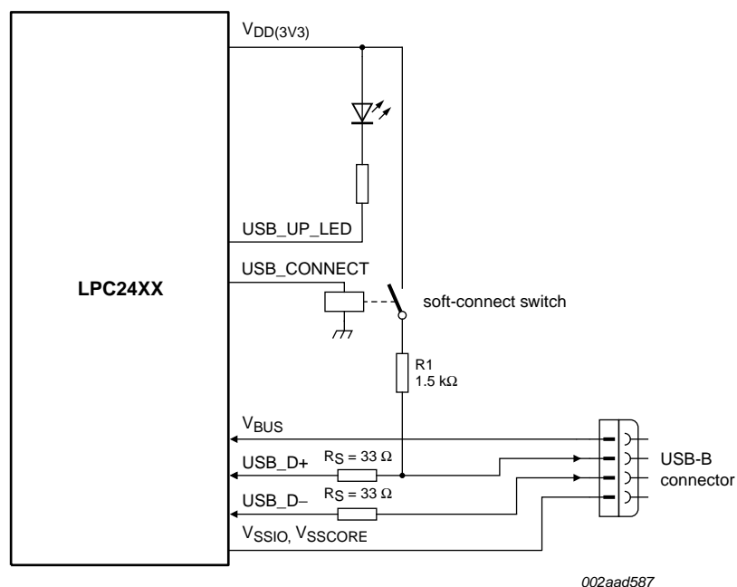
Fig 23. LPC2420/2460 USB interface on a self-powered device
