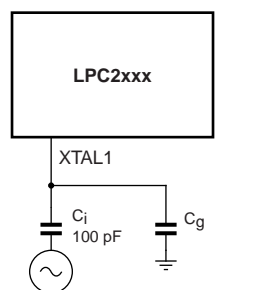
Fig 22. Slave mode operation of the on-chip oscillator
