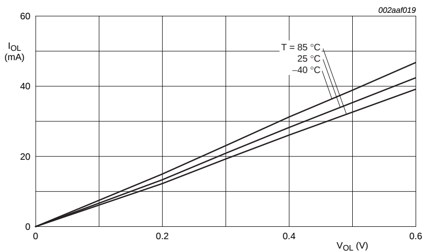
Fig 15. I 2 C-bus pins (high current sink): Typical LOW-level output current I_{OL} versus LOW-level output voltage V_{OL} .
