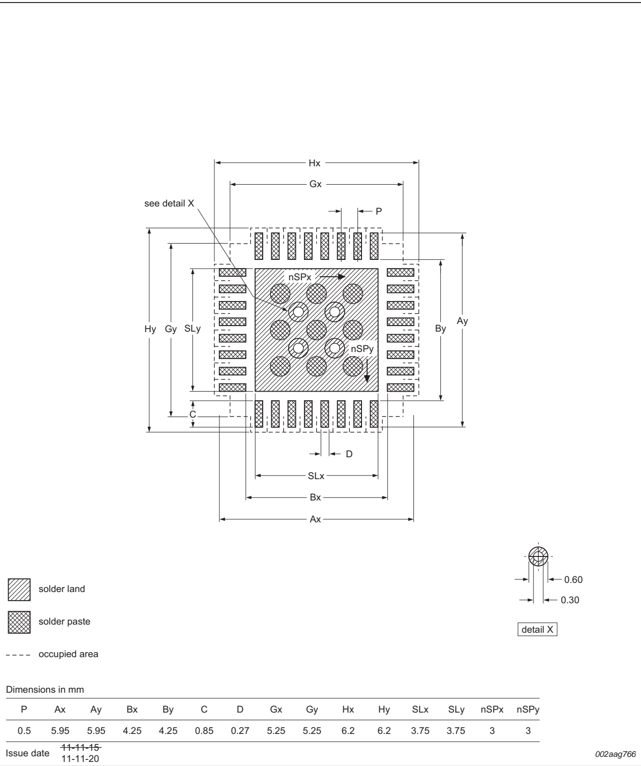
Fig 33. Reflow soldering for the HVQFN33 (5x5) package
