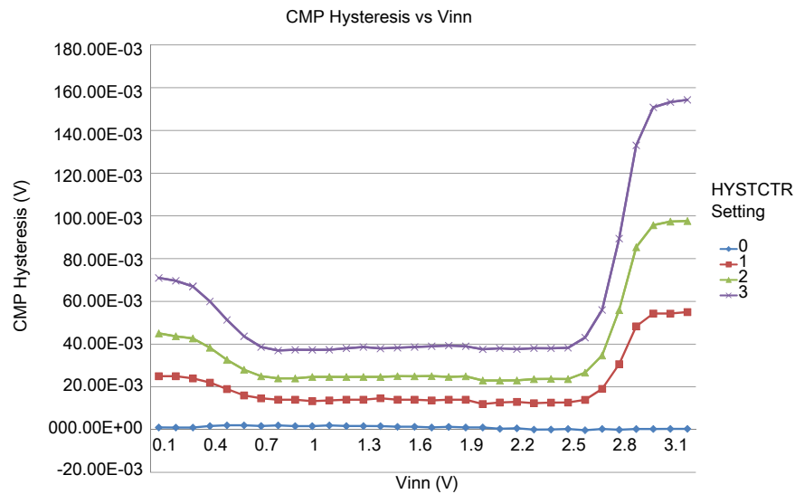
Figure 13. Typical hysteresis vs. Vin level ( V_{DD} = 3.3 \text{ V} , \text{PMODE} = 1 )
