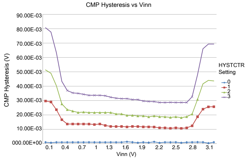
Figure 12. Typical hysteresis vs. Vin level ( V_{DD} = 3.3 \text{ V} , \text{PMODE} = 0 )
