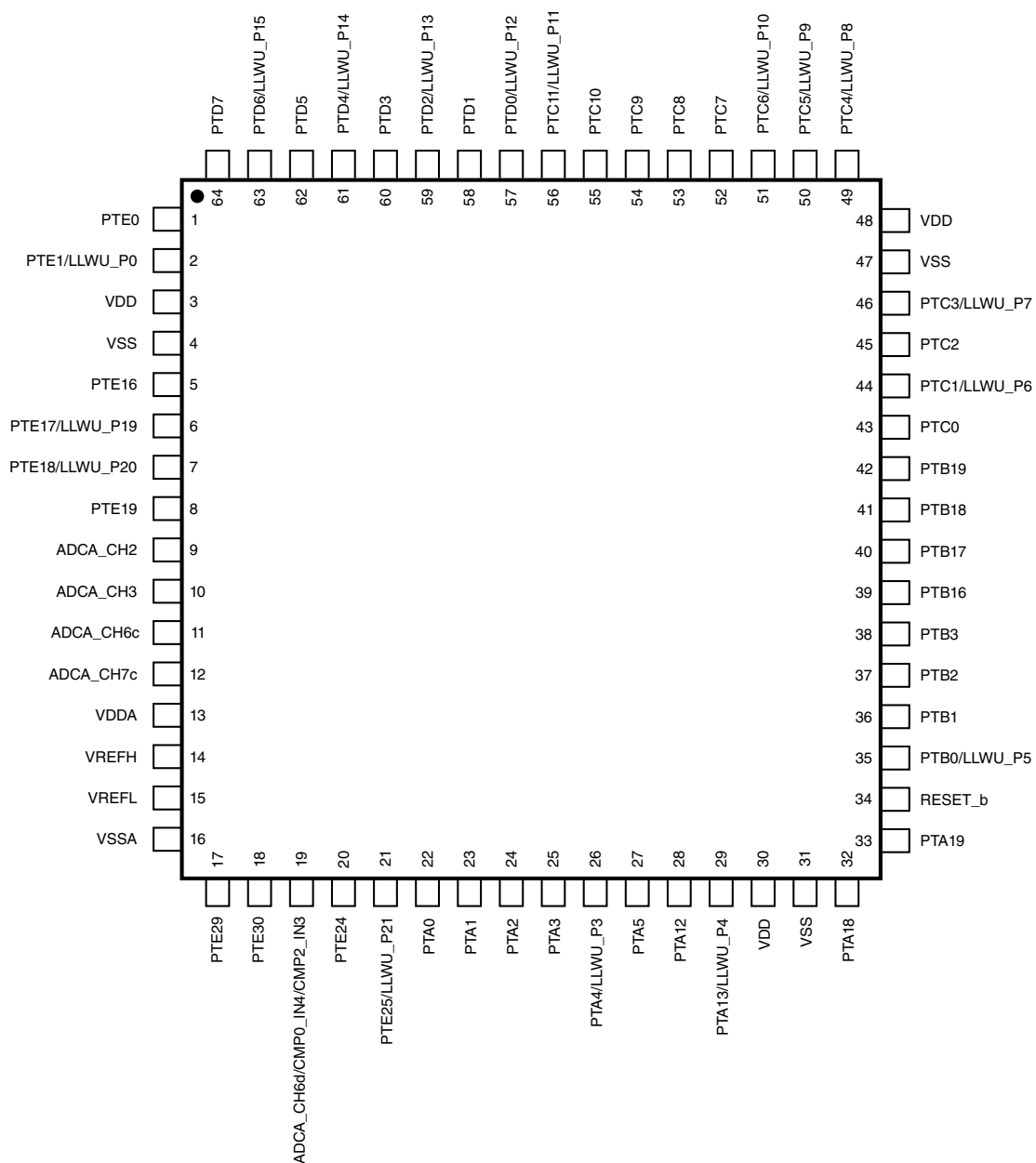
Figure 21. 64-pin LQFP
