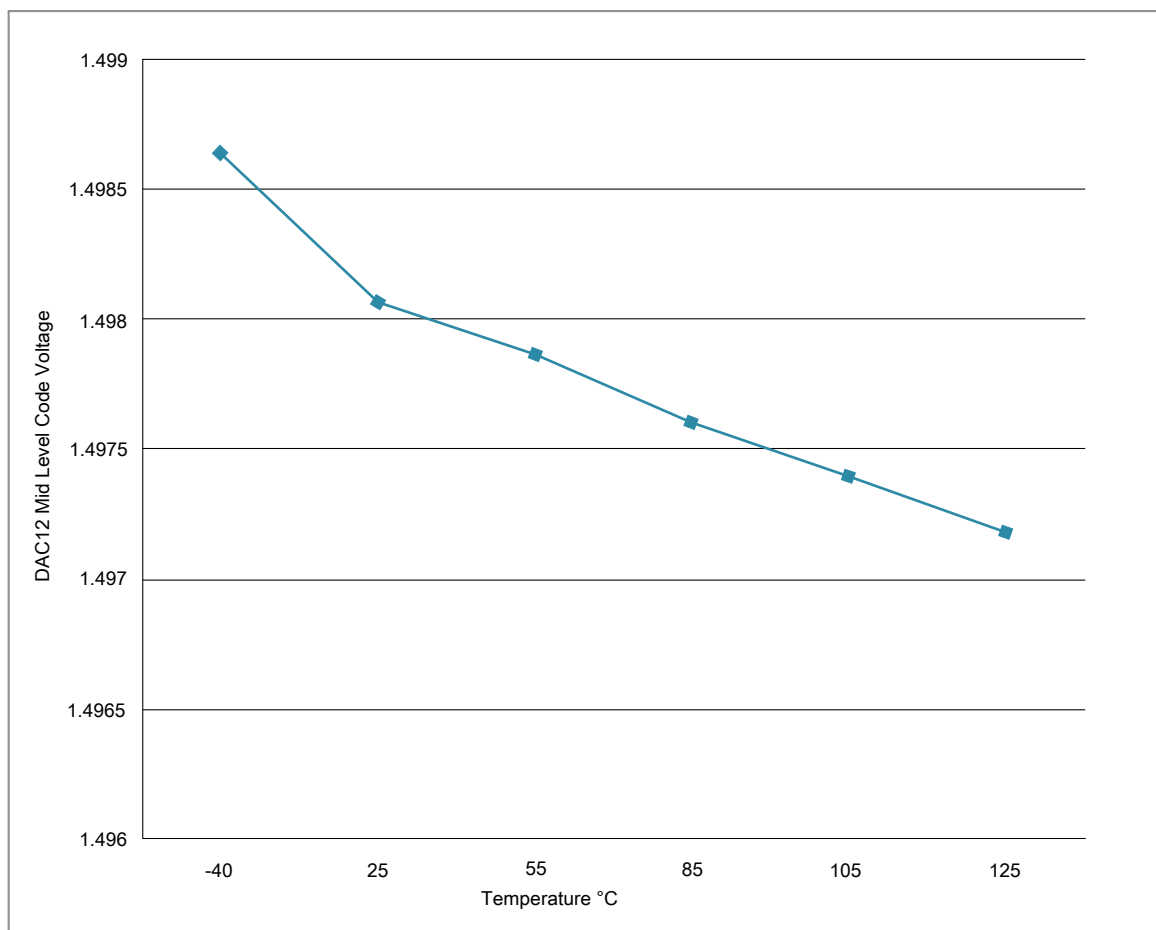
Figure 15. Offset at half scale vs. temperature
