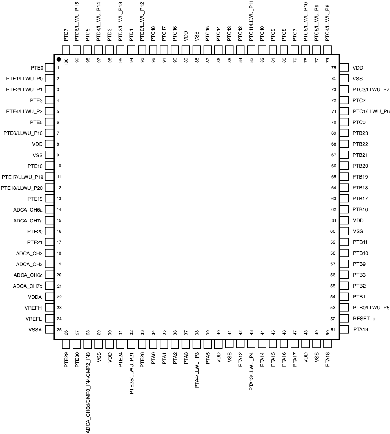
Figure 20. 100-pin LQFP
