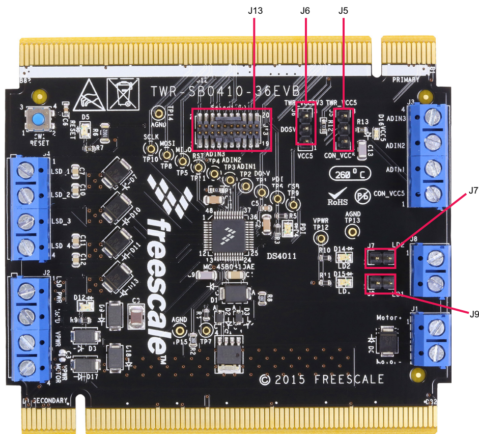
Figure 8. Jumper locations
