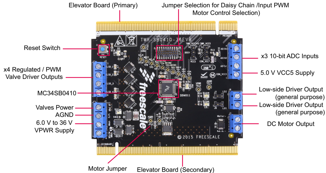
Figure 4. Board overview
