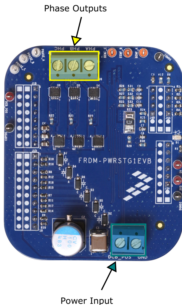
Figure 6. Screw terminals
