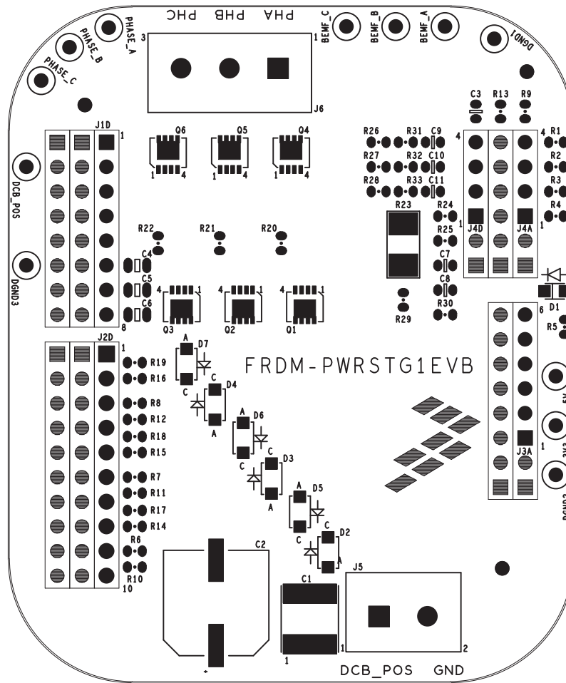
Figure 8. Silkscreen
