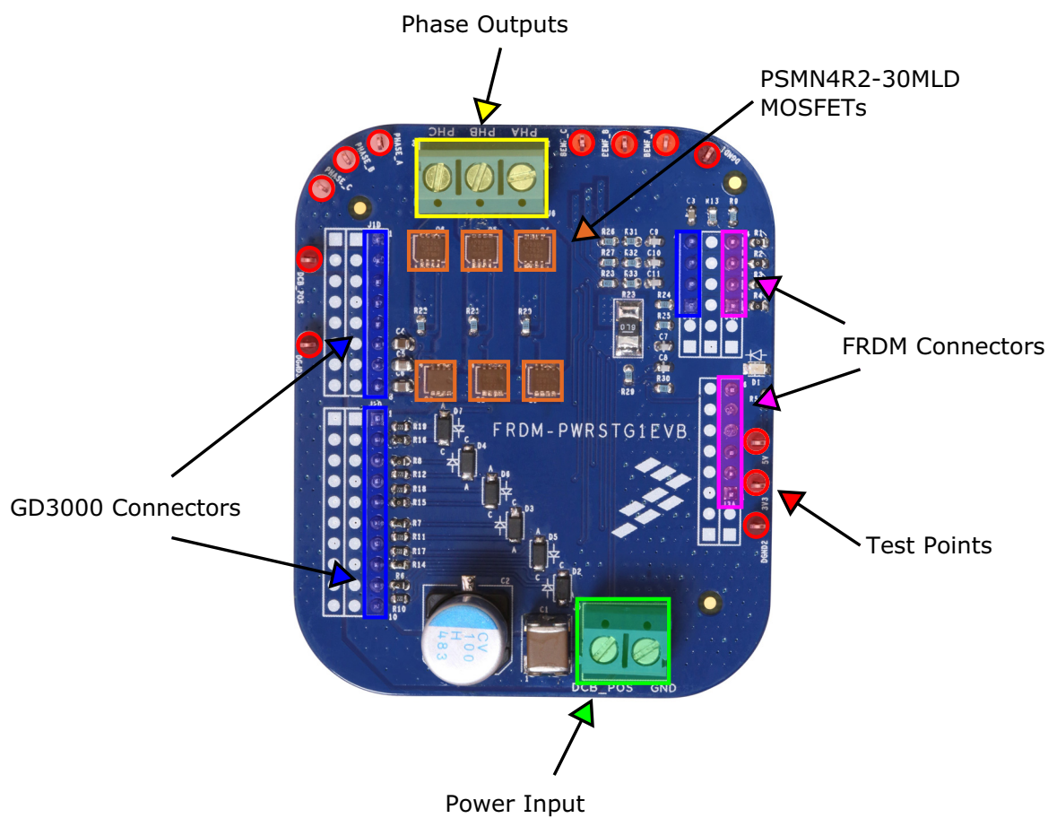
Figure 3. Board description
