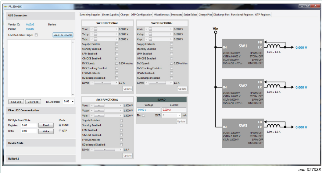
Figure 8. GUI startup
