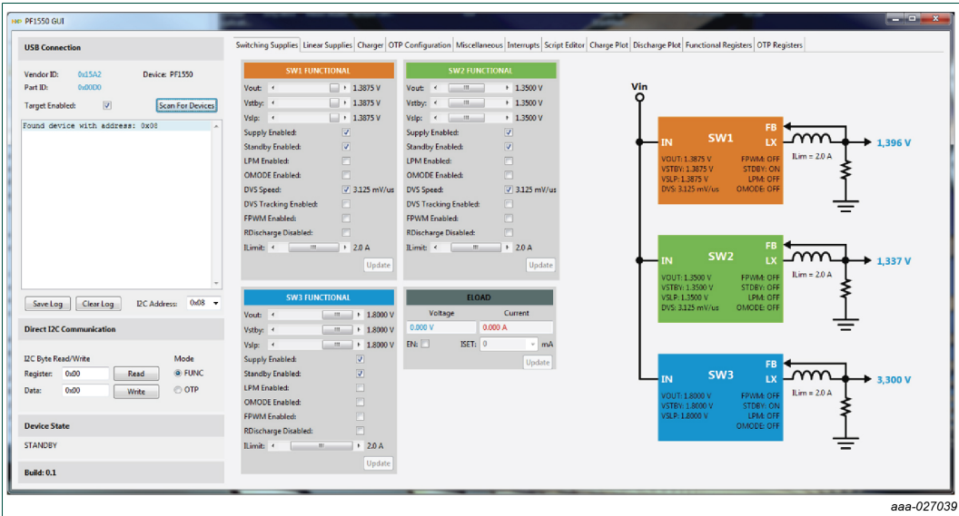
Figure 9. GUI connected to the target board
