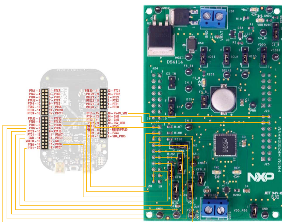
Figure 12. FRDM-KL25Z to FRDM-HB2000FEVM connections
