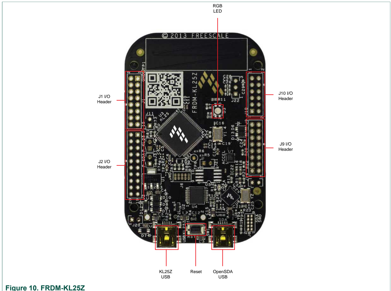
Figure 10. FRDM-KL25Z
