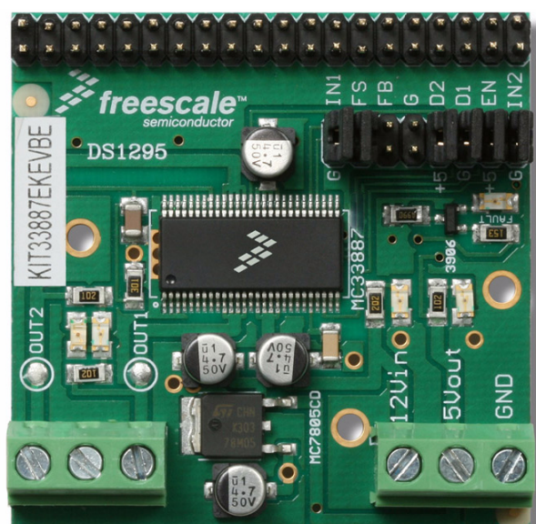
Figure 1. KIT33887EKEVB Evaluation Board
