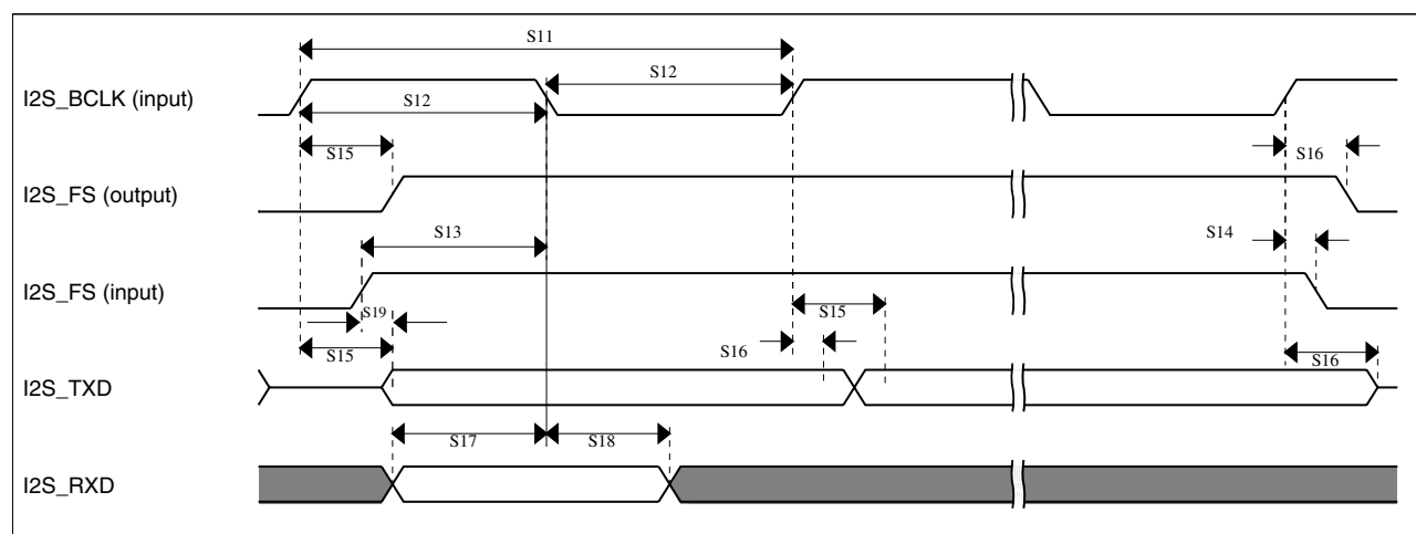
Figure 30. I 2 S timing — slave modes
