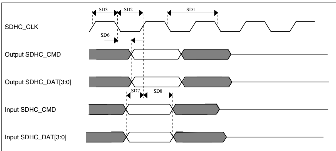
Figure 27. SDHC timing
