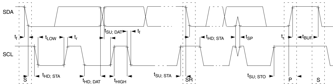
Figure 24. Timing definition for fast and standard mode devices on the I²C bus
