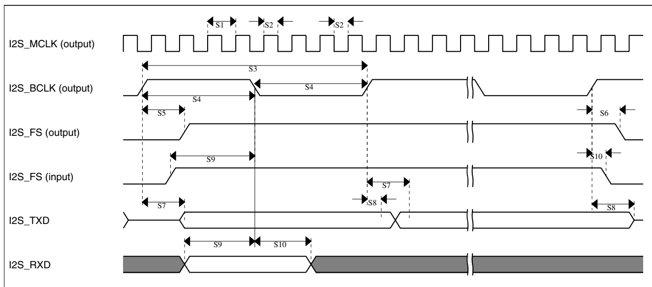
Figure 23. I²S timing — master mode
