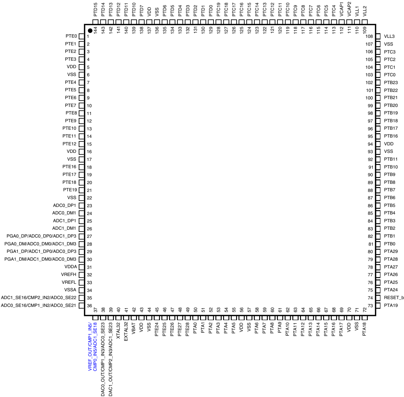
Figure 27. K30 144 LQFP Pinout Diagram
