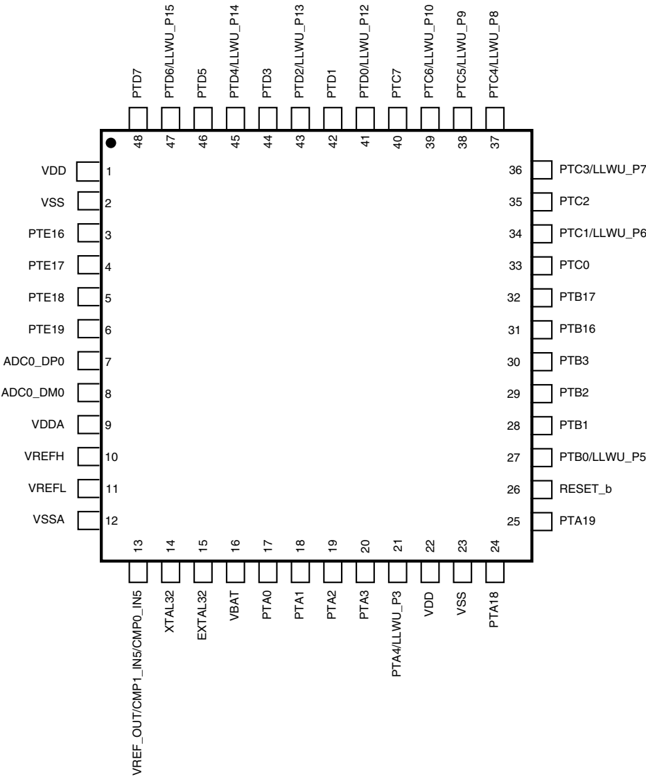
Figure 22. K12 48 LQFP Pinout Diagram
