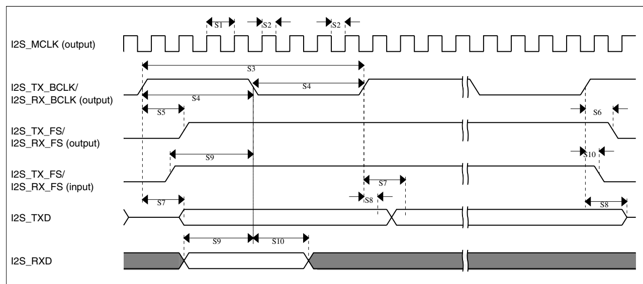
Figure 23. I2S/SAI timing — master modes
