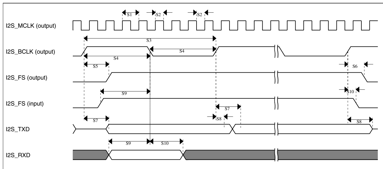
Figure 26. I²S timing — master mode
