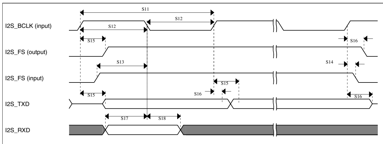
Figure 27. I²S timing — slave modes
