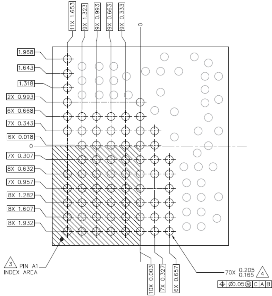
DETAIL E (I) (ARRAY BUMPS (70X))
