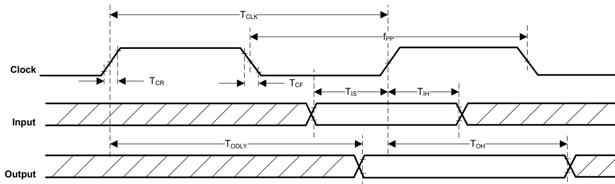
Figure 17. SDIO protocol timing diagram—SDR12, SDR25, SDR50 Modes (up to 100 MHz) (1.8V)
