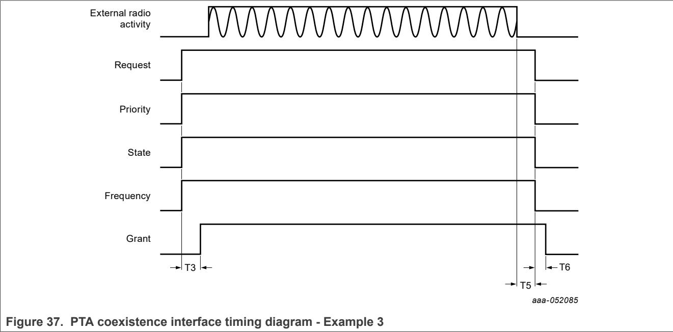
Figure 37. PTA coexistence interface timing diagram - Example 3
