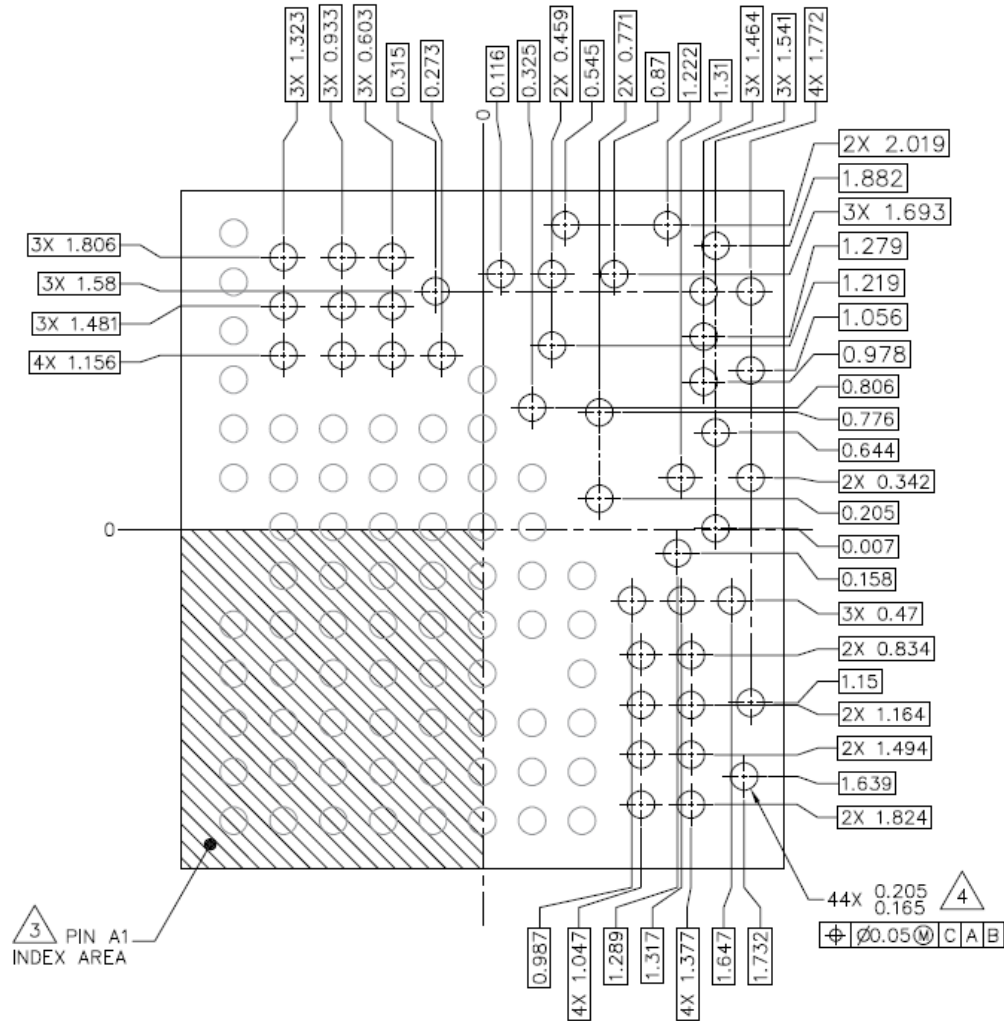
DETAIL E (II) (NON-ARRAY BUMPS (44X))
