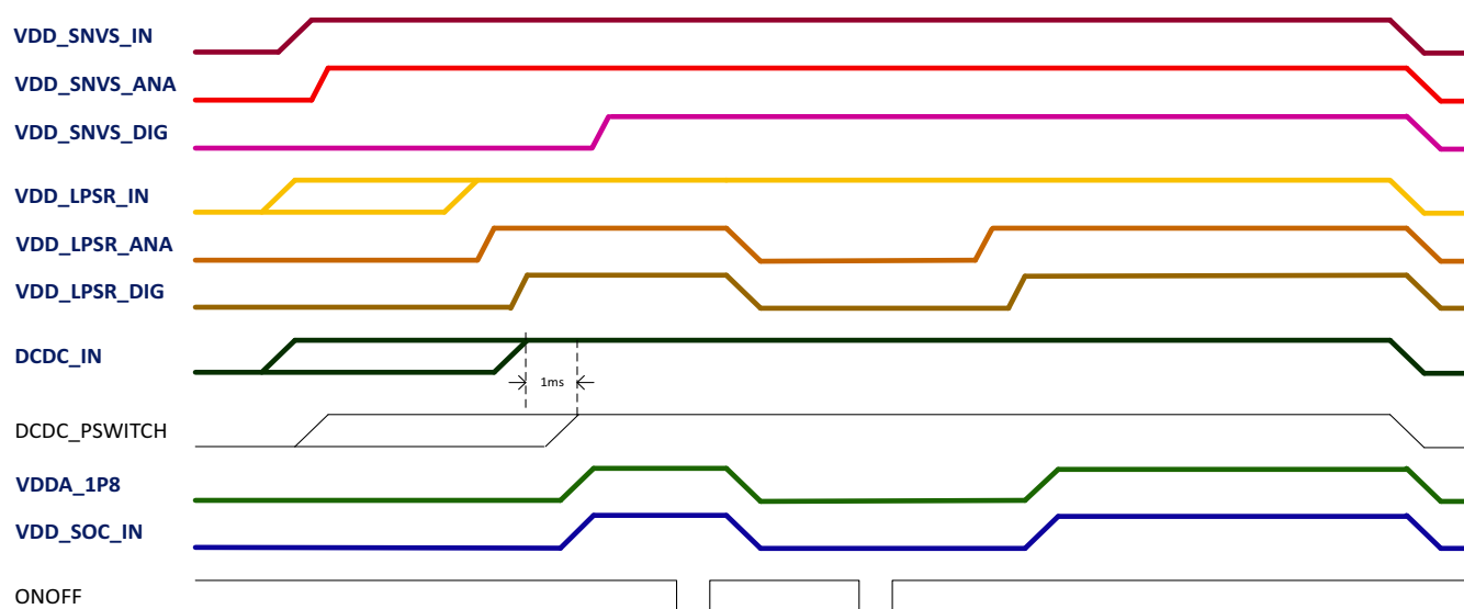
Figure 4. Power sequence
