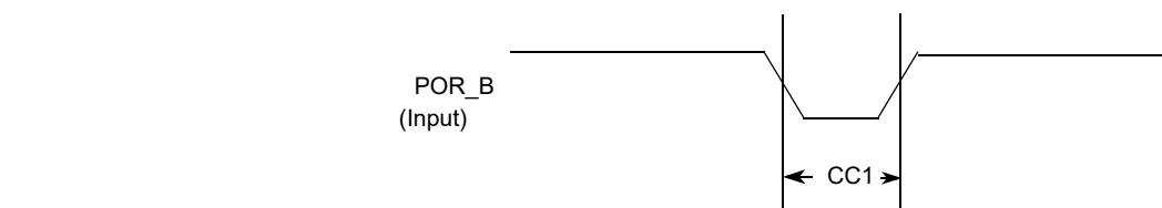
Figure 9. POR reset timing diagram
