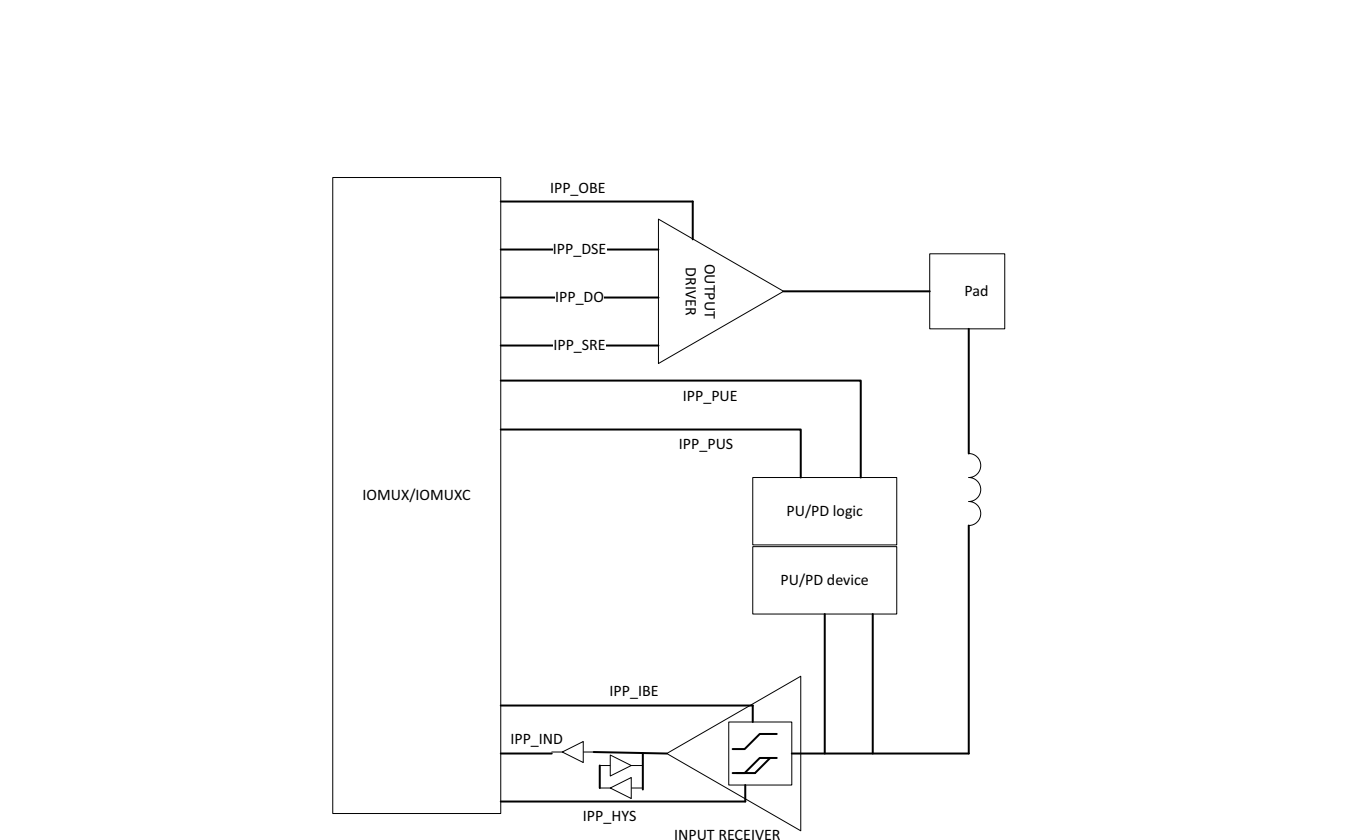
Figure 8. GPIO block diagram
