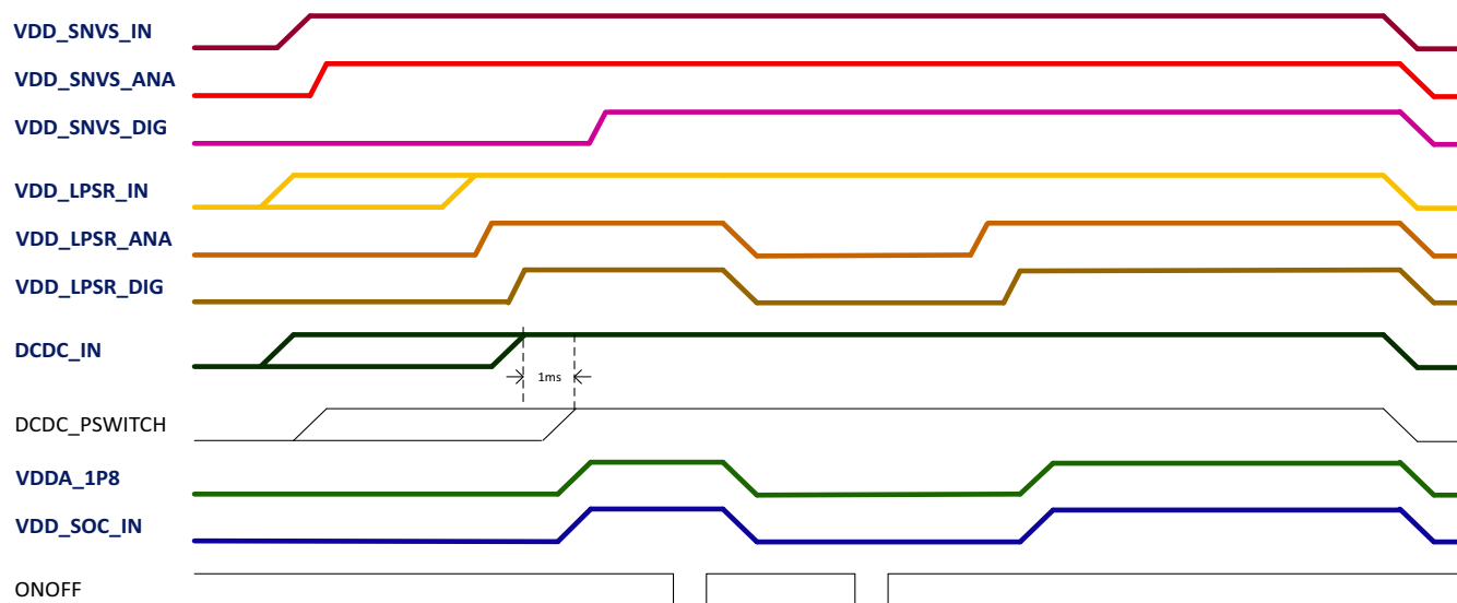
Figure 4. Power sequence
