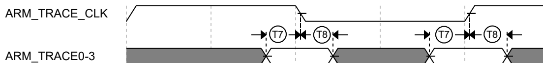
Figure 14. Trace data specifications
