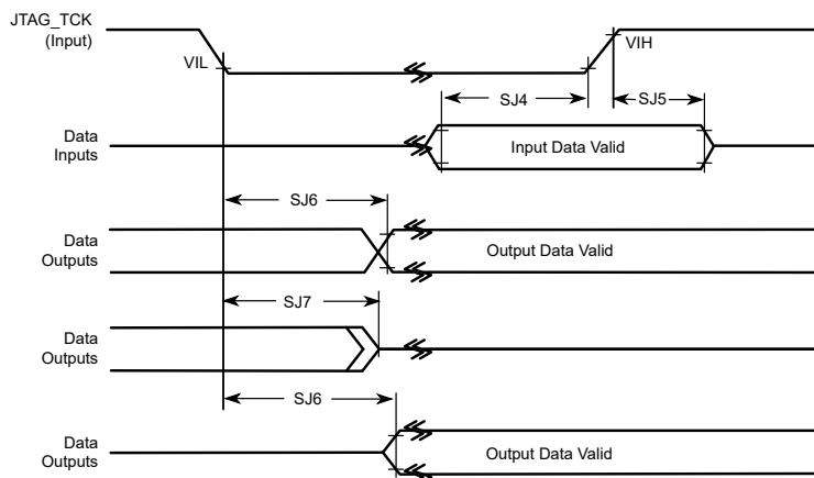
Figure 10. Boundary Scan (JTAG) timing diagram
