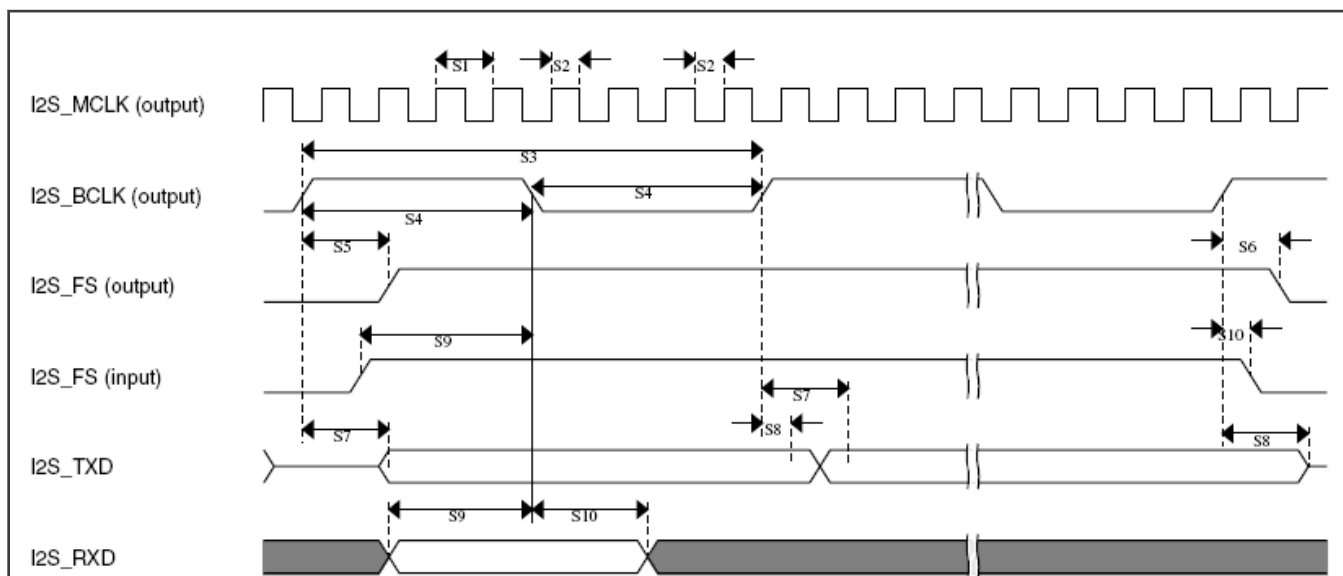
Figure 31. SAI timing—Master modes
