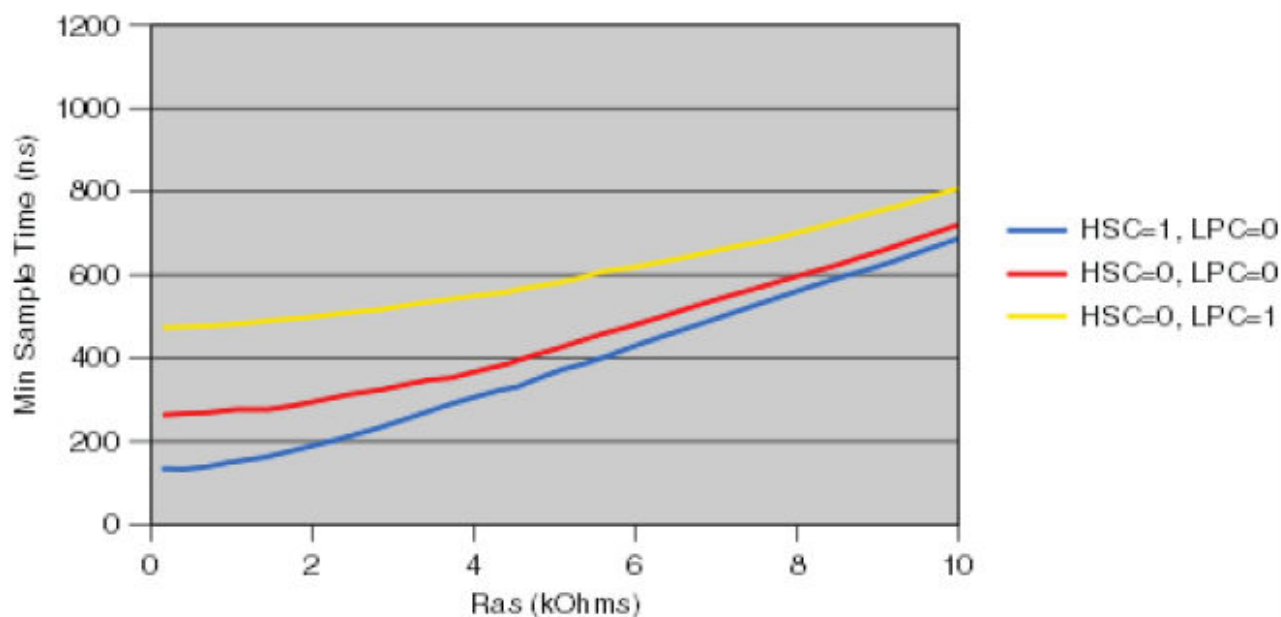
Figure 36. Minimum Sample Time Vs Ras (Cas = 2pF)
