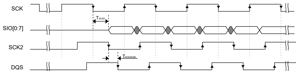
Figure 24. FlexSPI input timing in DDR mode where FlexSPIn_MCR0[RXCLKSRC] = 0x3 (case B2)
