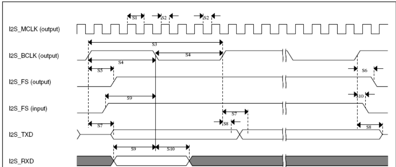
Figure 31. SAI timing—Master modes
