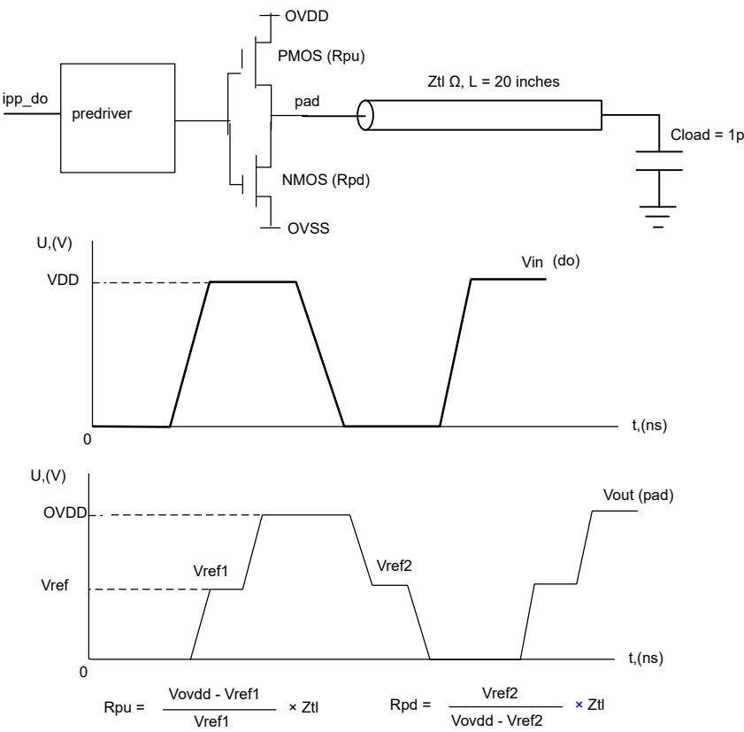
Figure 6. Impedance matching load for measurement
