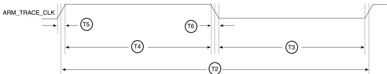
Figure 13. ARM_TRACE_CLK specifications
