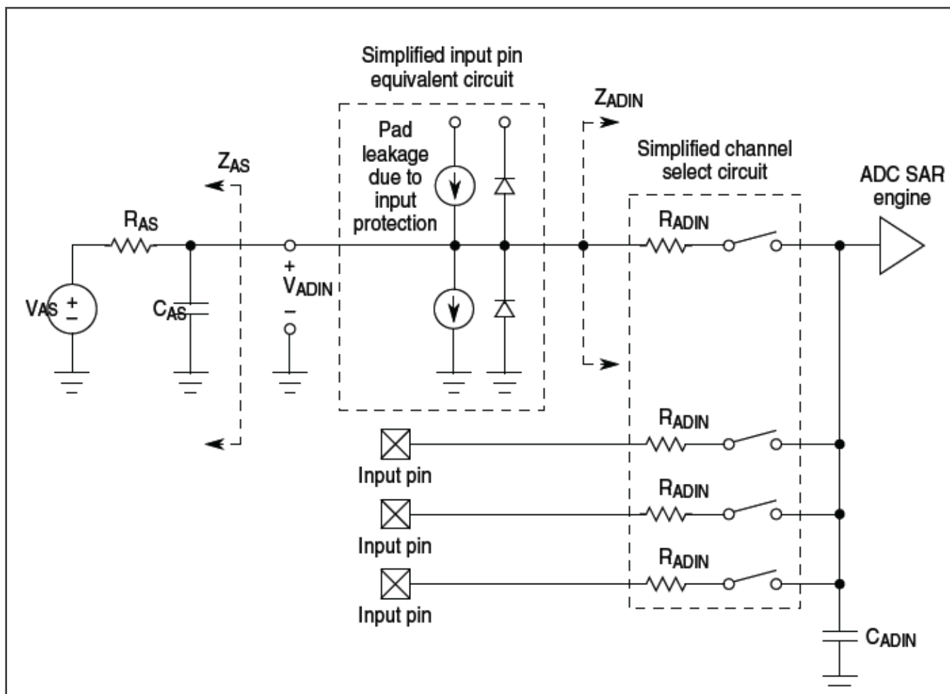
Figure 32. 12-bit ADC input impedance equivalency diagram
