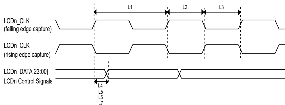
Figure 27. LCD timing
