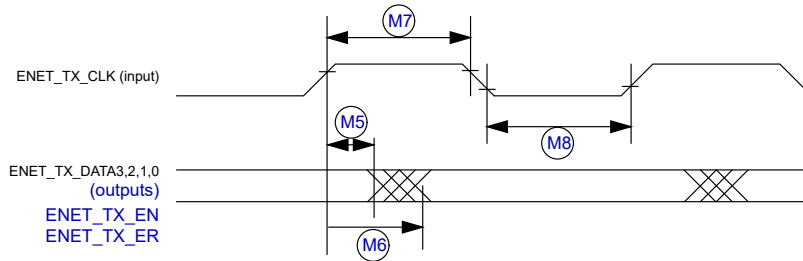
Figure 45. MII transmit signal timing diagram
