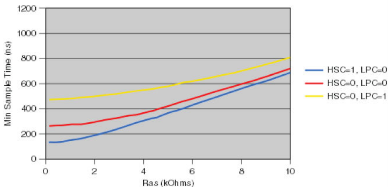
Figure 33. Minimum Sample Time Vs Ras (Cas = 2pF)
