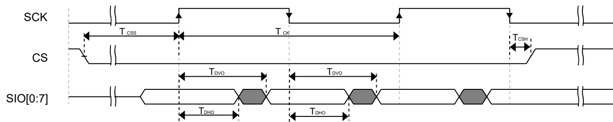
Figure 26. FlexSPI output timing in DDR mode
