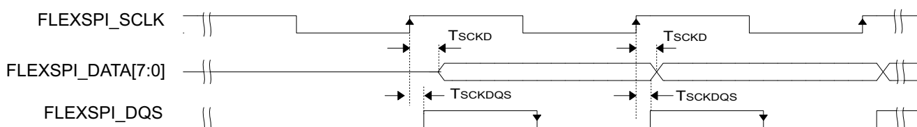
Figure 45. FlexSPI input timing in SDR mode where FlexSPI IN _MCR0[RXCLKSRC] = 0X3 (case A1)
