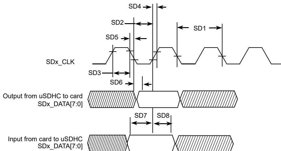
Figure 22. SD3.0/eMMC5.1 (SDR) timing
