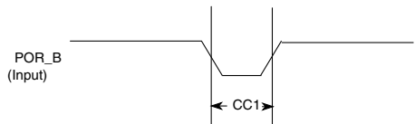
Figure 10. Reset timing diagram
