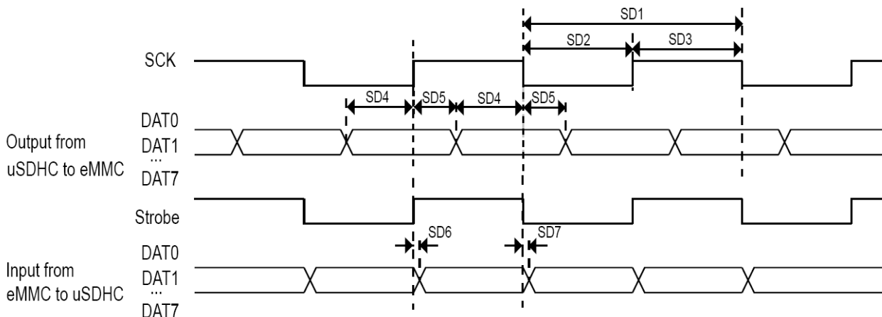
Figure 30. HS400 timing
