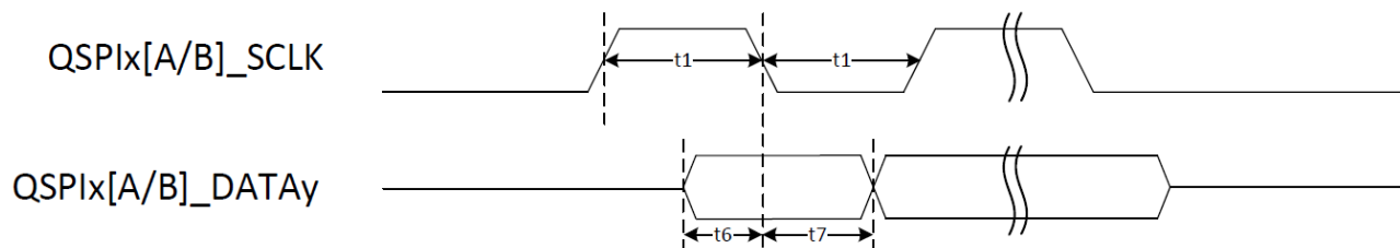
Figure 42. FlexSPI read timing diagram (SDR mode)
