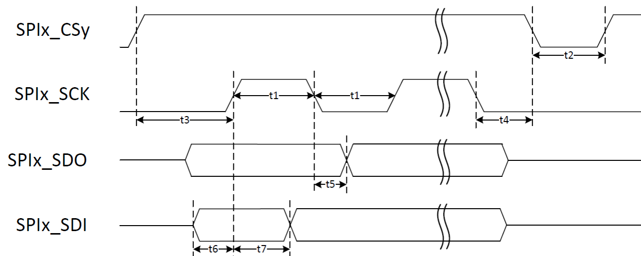
Figure 23. LPSPI Master mode
