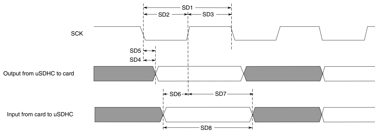
Figure 32. SDR50/SDR104 timing
