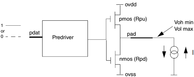
Figure 4. Circuit for Parameters Voh and Vol for I/O Cells
