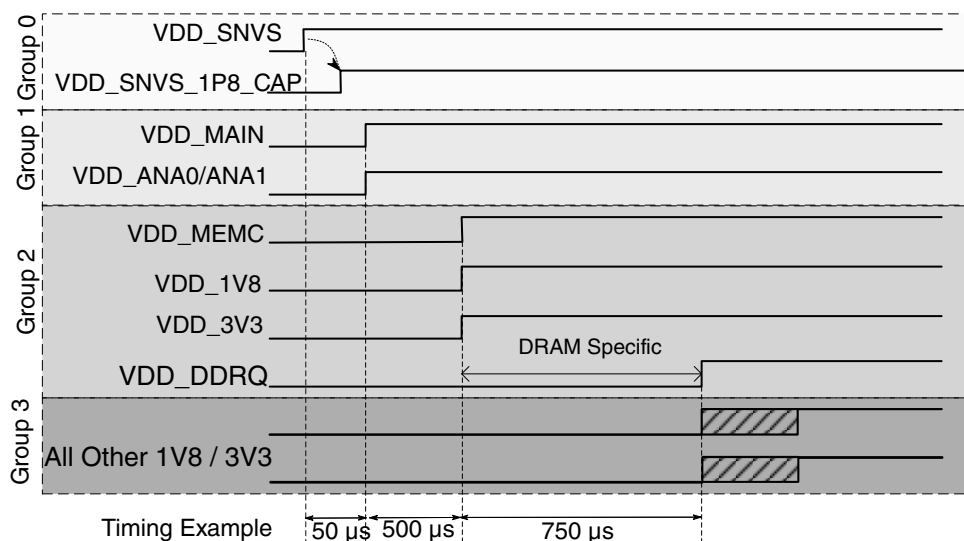
Figure 3. Power-up Timing Diagram
