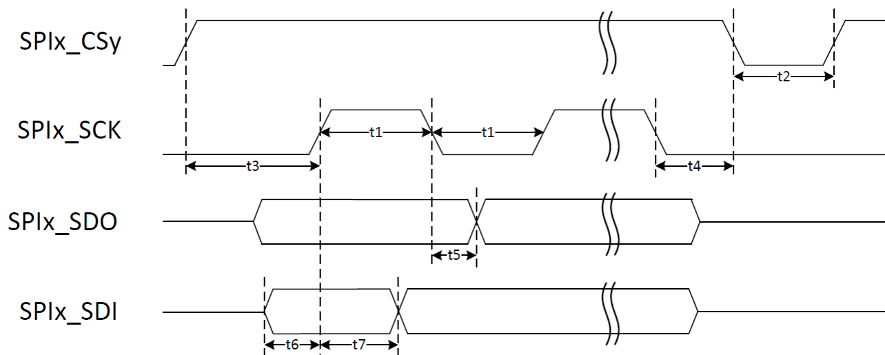
Figure 24. LPSPi Slave mode
