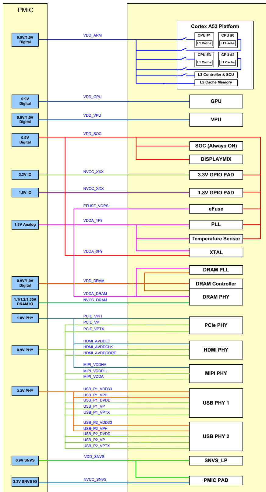
Figure 3. Power architecture
