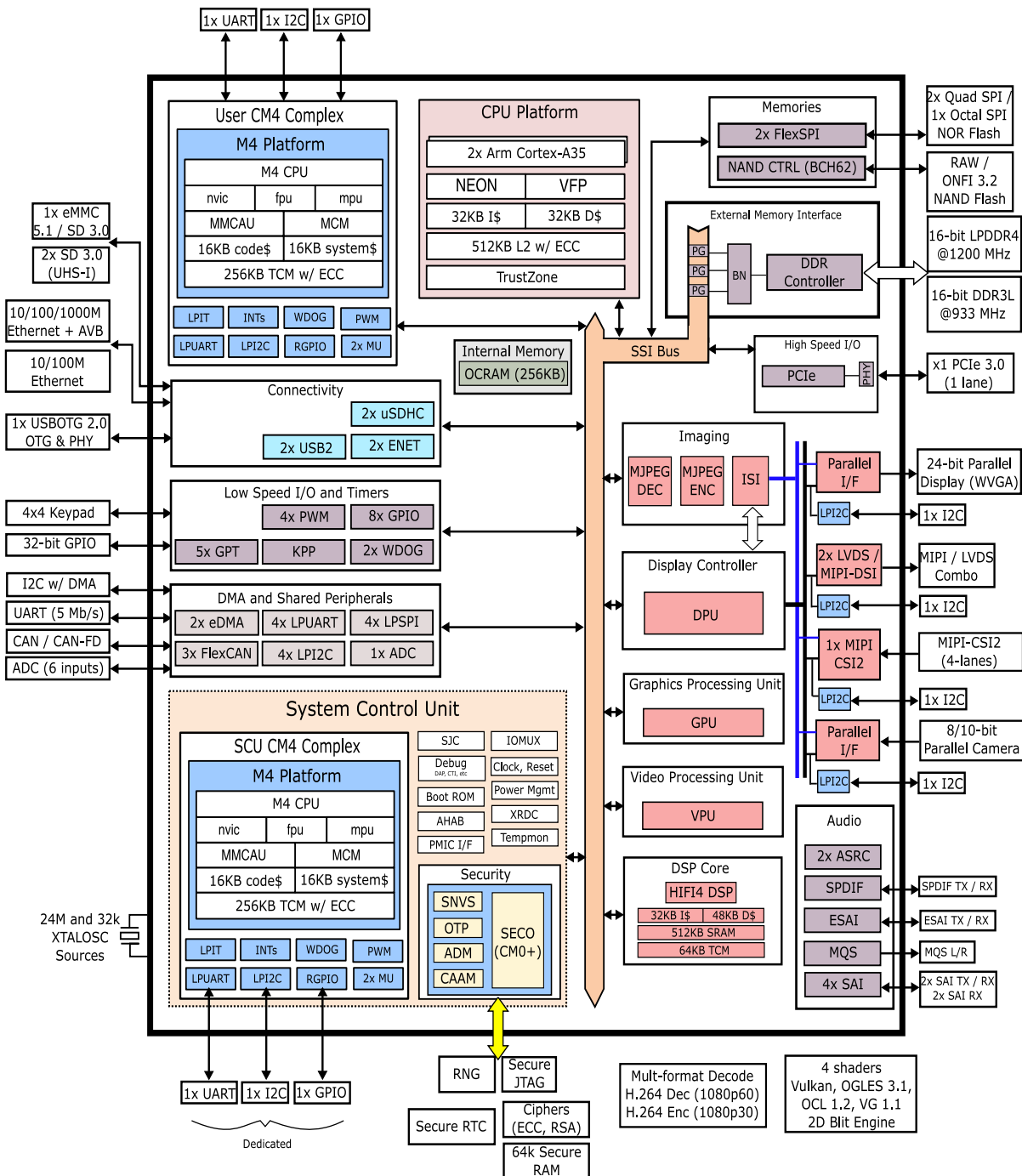
Figure 1. i.MX 8DualX System Block Diagram
