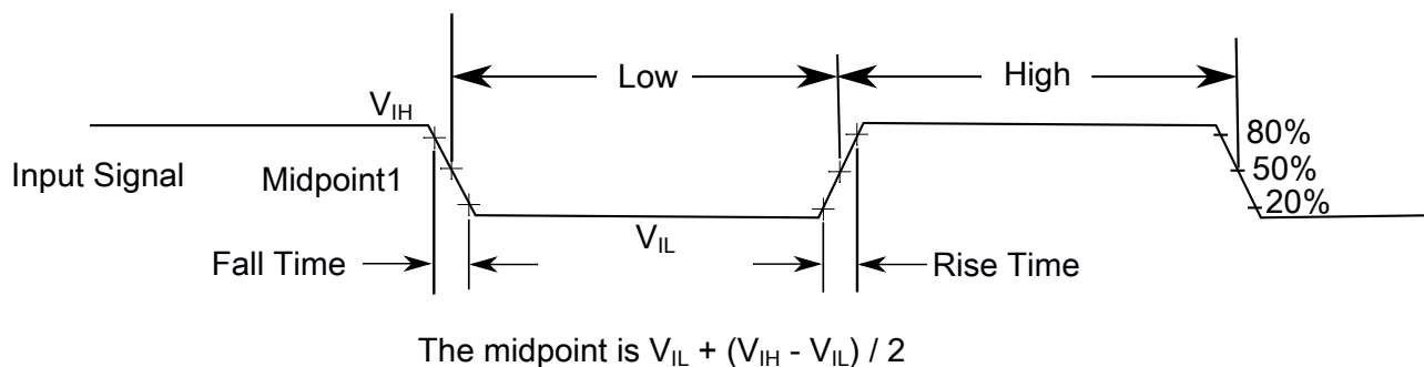
Figure 4. Input signal measurement reference
