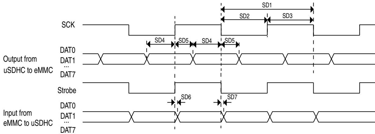
Figure 14. HS400 timing
