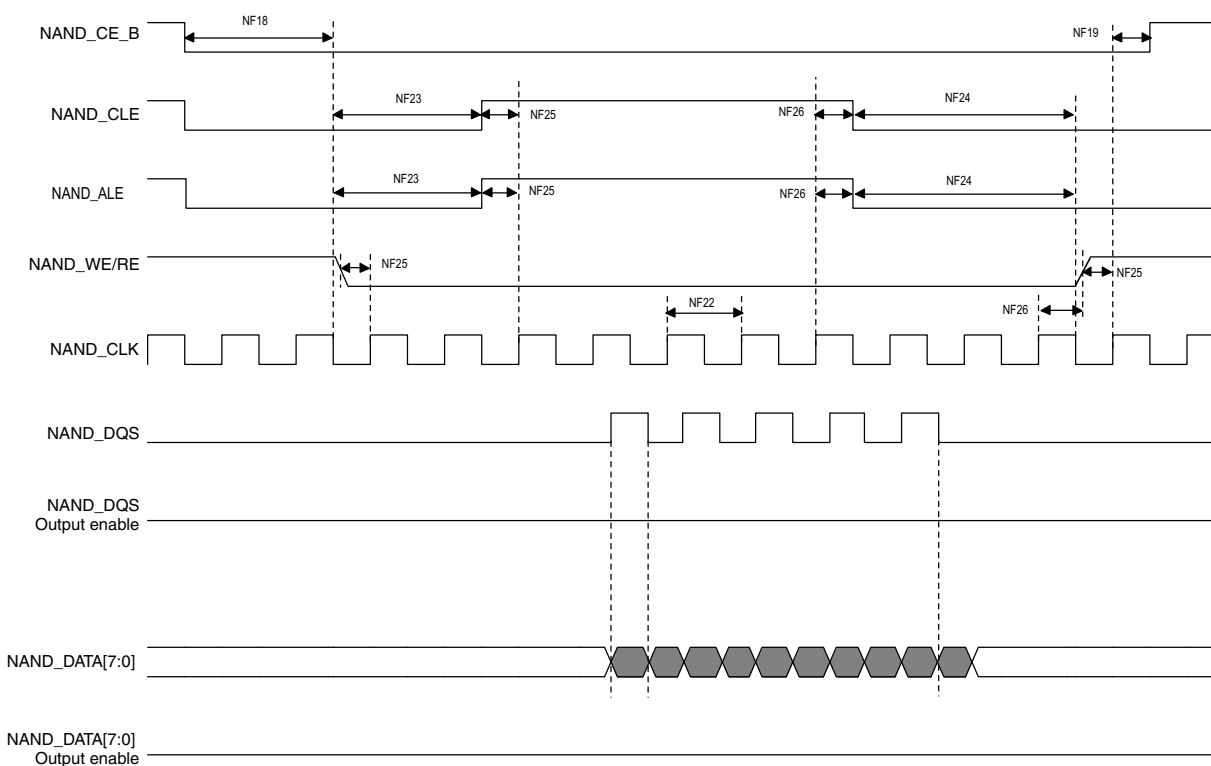
Figure 29. Source Synchronous Mode Data Read Timing Diagram
