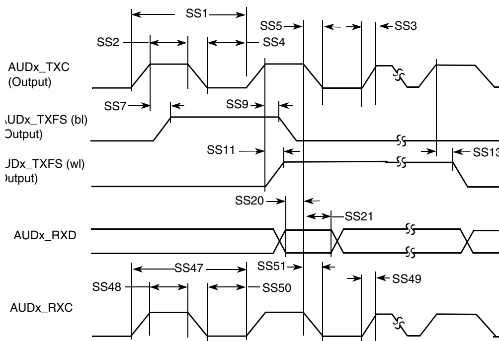
Figure 32. SSI Receiver Internal Clock Timing Diagram
