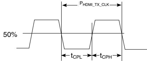
Figure 52. TMD5 Clock Signal Definitions
