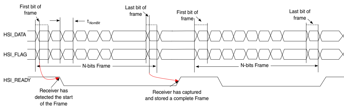
Figure 72. Synchronized Data Flow READY Signal Timing (Frame and Stream Transmission)
