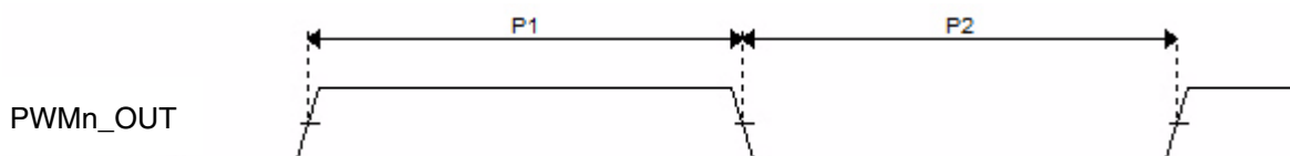
Figure 79. PWM Timing
