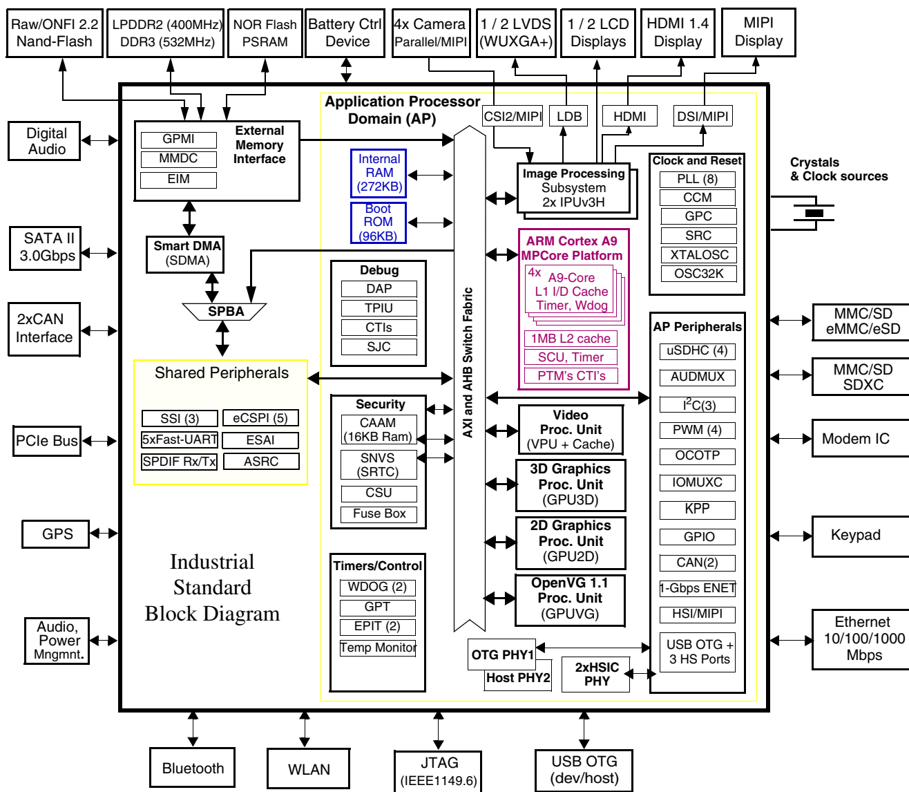
Figure 2. i.MX 6Dual/6Quad Industrial Grade System Block Diagram
