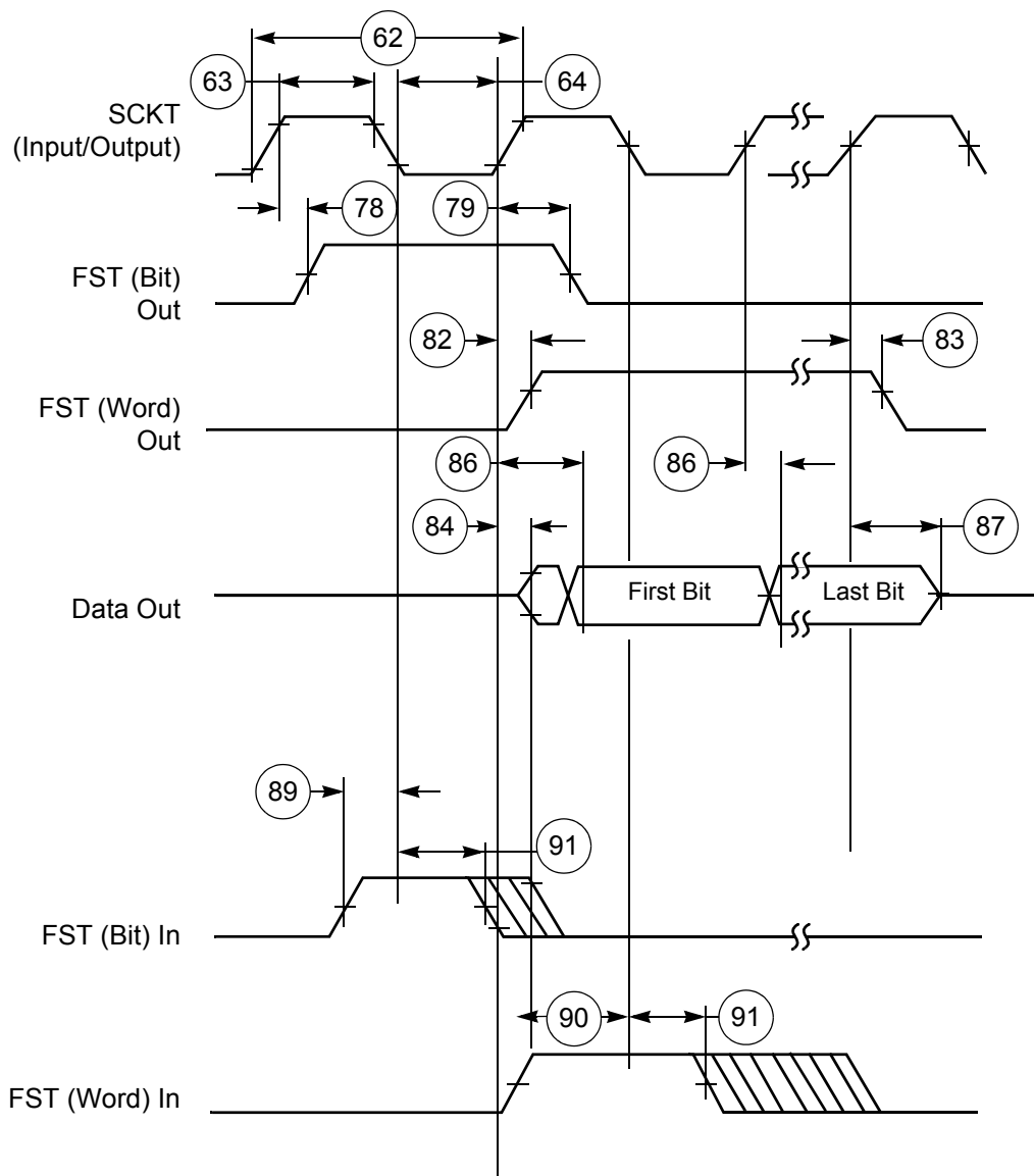
Figure 34. ESAL Transmitter Timing
