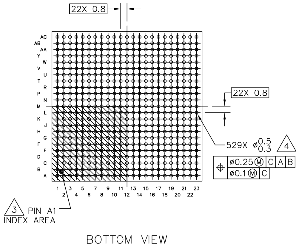
Figure 101. 19 x 19 mm Package, 529 Solder Balls, Bottom View
