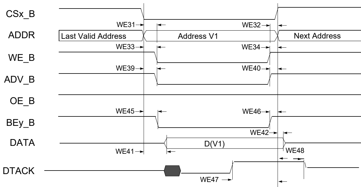
Figure 27. DTACK Write Access (DAP=0)
