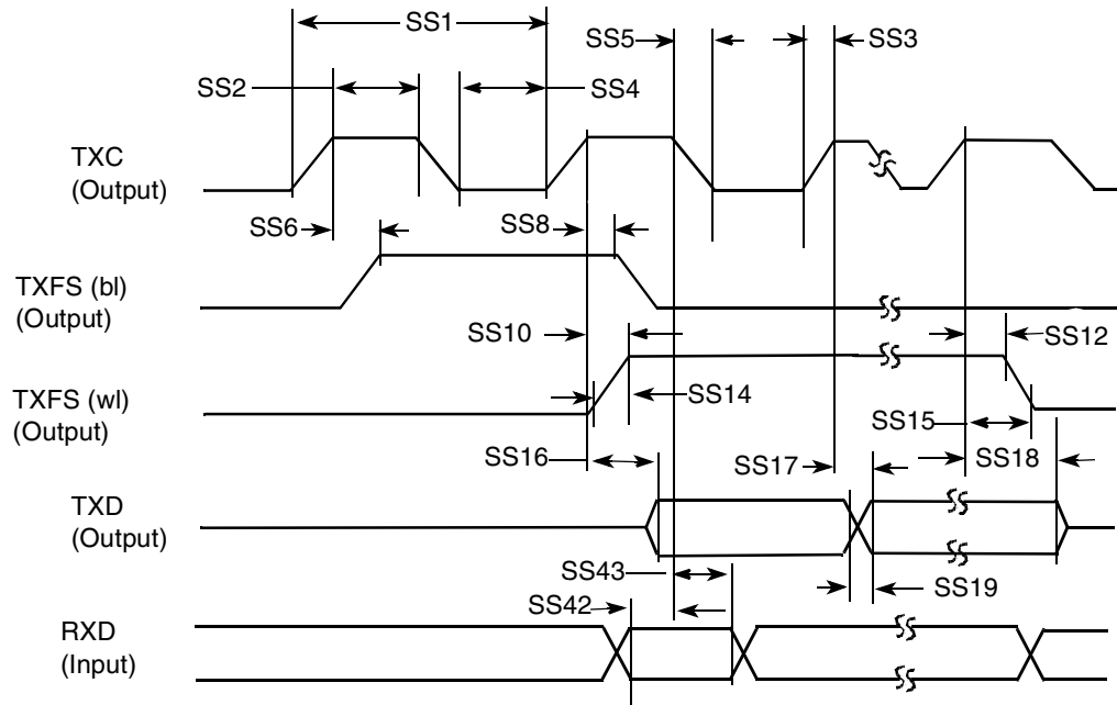
Figure 92. SSI Transmitter Internal Clock Timing Diagram
