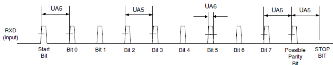
Figure 99. UART IrDA Mode Receive Timing Diagram
