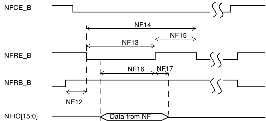
Figure 17. Read Data Latch Timing—Asymmetric Mode
