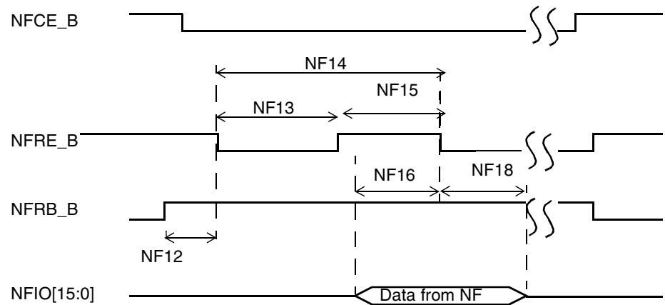
Figure 18. Read Data Latch Timing—Symmetric Mode
